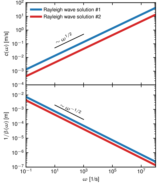
FIG. 7. Traditional Rayleigh wave solutions at the vacuum-water interface. The dispersion relation for the traditional Rayleigh wave Eq. (34) is solved numerically to obtain the wave number k as a function of \omega . Phase velocities and propagation distances are obtained from k(\omega) via Eqs. (15), (16).
