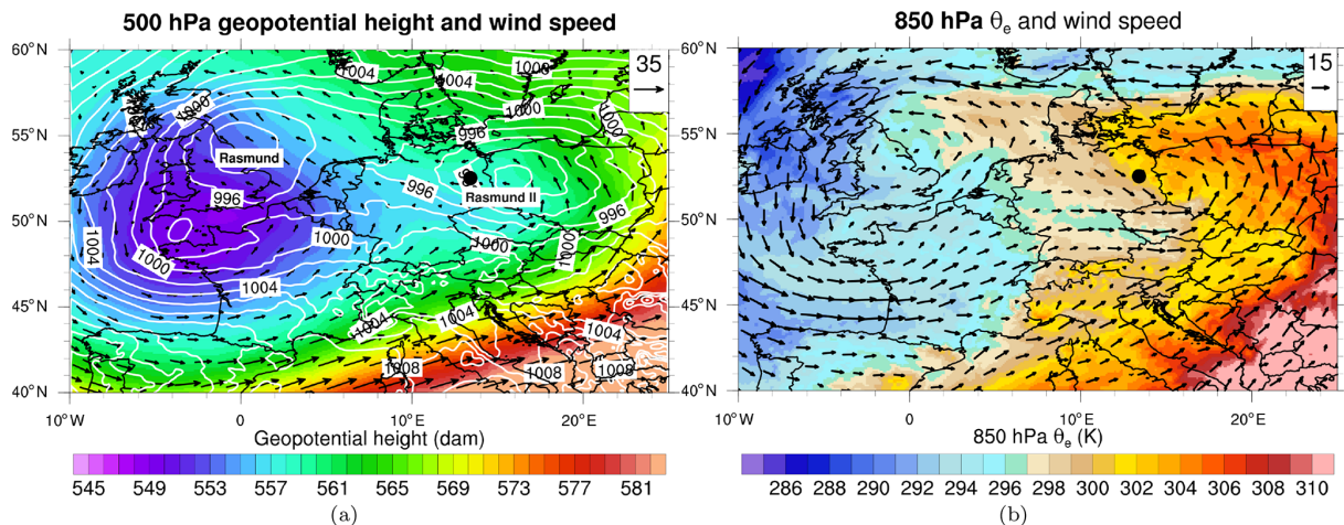
Figure 3. (a) 500 hPa geopotential height (dam; colour) and wind speed ( \text{ms}^{-1} ) together with sea level pressure (hPa; contours) and (b) 850 hPa equivalent potential temperature ( \theta_e ) and wind speed on 29 June 2017 12:00 UTC from the ECMWF analysis. The black dot denotes the city of Berlin.
