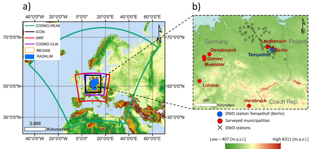
Figure 1. (a) Spatial extent of the used data sets REGNIE, RADKLIM, COSMO-REA6, WRF-1.5 km, ICON-625 m and COSMO-CLM-2.8. (b) Close-up view of Berlin and surroundings, and the DWD stations used for validation (crosses), the location of surveyed events from Table 1 (red dots) and the Berlin–Tempelhof station analysed in Fig. 11 (blue dot), basemap: Global Land One-kilometer Base Elevation (GLOBE) (Hastings et al., 1999).
