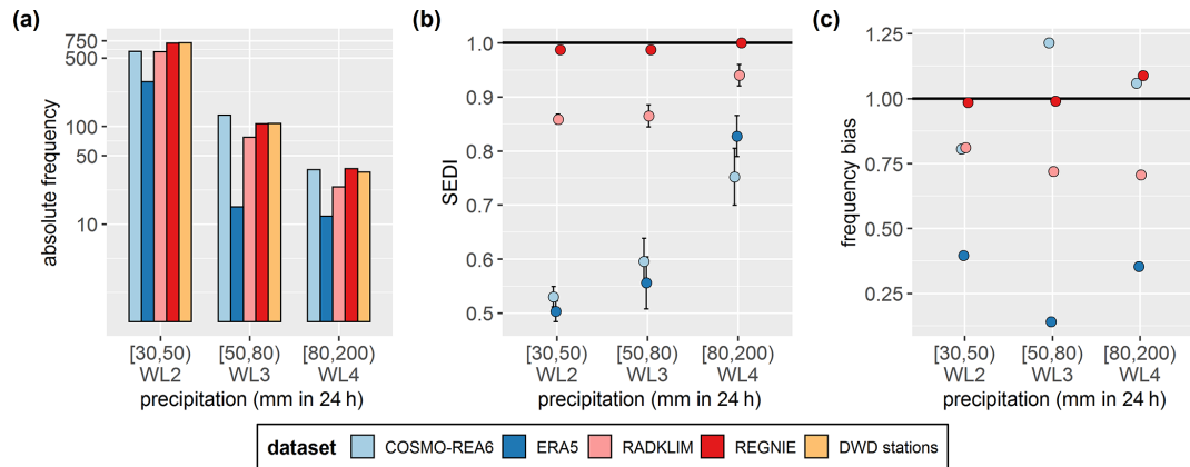
Figure 2. Evaluation of daily precipitation estimates from REGNIE, RADKLIM, ERA5 and COSMO-REA6 compared with DWD station observations (see Fig. 1b). The selected period is 2001 to 2018 (concurrent period of data availability), using the nearest neighbour grid cells to the DWD stations. (a) Histogram showing the absolute occurrences of precipitation within WLS 2, 3 and 4, (b) symmetric extremal dependency index (SEDI) and (c) frequency bias. Positive (negative) frequency bias indicates an overestimation (underestimation) of events, the black horizontal line represents the optimum value.
