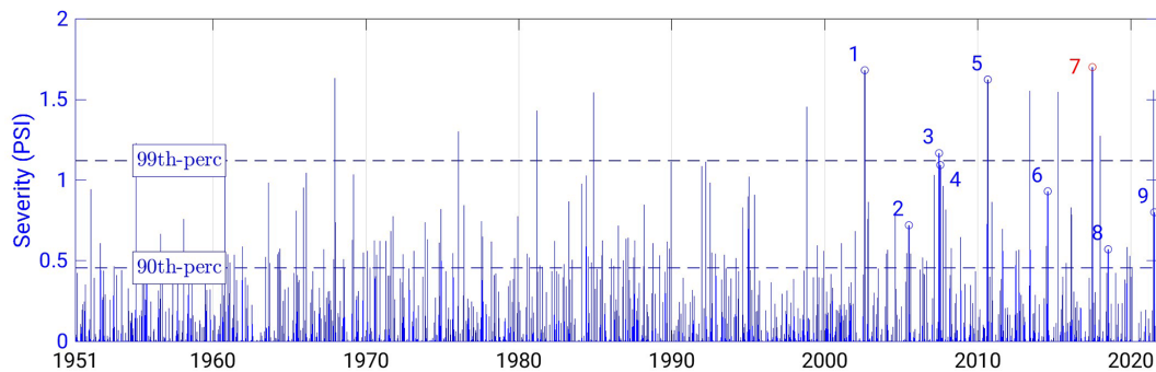
Figure 6. Temporal evolution of the PSI (blue bars) for the time period 1951 to 2021. The results are based on REGNIE daily precipitation observations between January 1951 and September 2021. The 99th percentile and 90th percentile of daily PSI values are represented by the dashed blue horizontal lines. Numbered circles highlight nine events analysed in Table 1 or in Fig. 7 and other historical events. These are (1) the Saxony floodings on the 12 August 2002; (2) the 29 June 2005 event, affecting Hersbruch and Lohmar; (3) the 21 June 2007 and the (4) 22 July 2007 events affecting Germany in its totality; (5) the 26 August 2010 event in Osnabrueck; (6) the 29 July 2014 event in Muenster and Greven; (7) the 29 June 2017 HPE (red); (8) the 12 July 2018 causing flooding in Berlin; and (9) the Ahr flooding on 14 July 2021.
