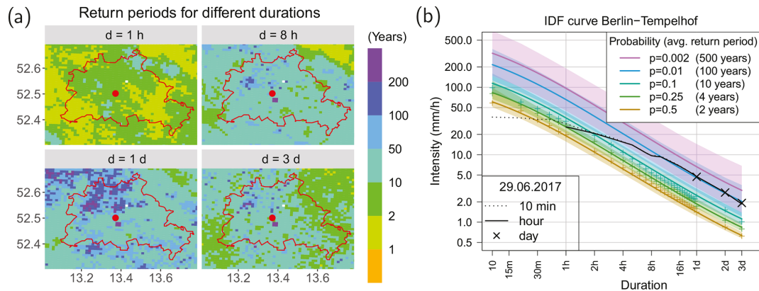
Figure 11. (a) Return periods of this event’s intensity from gridded RADKLIM (1 km \times 1 km) data using a duration-dependent GEV distribution. Red dot: position of DWD weather station Tempelhof used to construct the IDF curve in (b). (b) IDF curves from station-based data. The coloured lines show return periods from the d -GEV model, the black line indicates intensity of the event on the 29 June for different temporal measurement resolutions. Empirical quantiles are denoted as coloured “+”. The 95 % confidence intervals come from 1000-fold bootstrapping.
