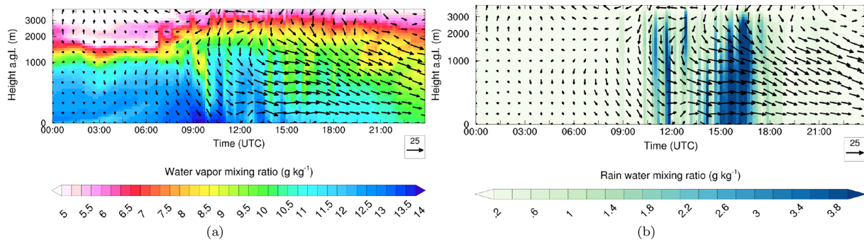
Figure 4. Time–height cross section of (a) water vapour mixing ratio ( \text{g kg}^{-1} ) and (b) rain water mixing ratio ( \text{g kg}^{-1} ) at grid point 13.2^\circ \text{ E} and 52.85^\circ \text{ N} (close to the maximum heavy precipitation location, near black dot in Fig. 3) simulated by the WRF model. The displayed period is 00:00 until 23:45 UTC on 29 June 2017. Arrows denote the horizontal wind speed ( \text{m s}^{-1} , see lower right of the plots for a length indicating 25 \text{ m s}^{-1} ) and direction at the different altitudes. Altitude is above ground level (AGL).
