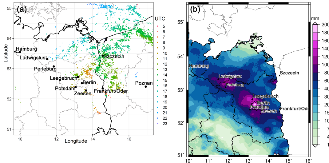
Figure 5. (a) Cloud-to-ground strokes from the EUCLID data set, colour-coded according to the time of occurrence from 05:00 UTC on 29 June 2017 to 00:00 UTC on the following day, and (b) 24 h precipitation totals (mm) during the study period (29 June 2017 06:00 UTC to 30 June 2017 06:00 UTC) from REGNIE.
