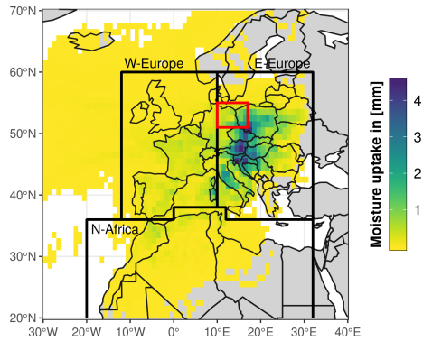
Figure 9. Moisture uptake within the planetary boundary layer, calculated based on Lagrangian backward trajectories using ERA5 reanalysis data. Hourly initialised trajectories on 29 June 2017 (00:00 to 23:00 UTC) at the region of heavy precipitation (red box) from 1000 to 200 hPa in steps of 50 hPa and 80 km horizontal distances, going back 240 h in time, are used to compute moisture uptake based on humidity changes, if they are associated with precipitation in the target region.
