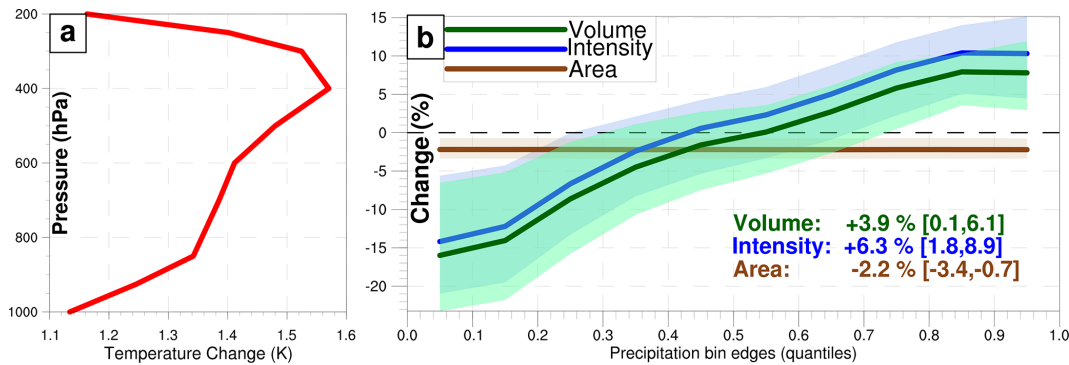
Figure 12. (a) Vertical warming signal and (b) response of event precipitation to warming signal. The warming is based on a subset of 17 CMIP6 models. The x axis in (b) shows precipitation bins which are delineated by quantiles of the precipitation intensity distribution; the changes in area and volume represent the changes associated with precipitation in these bins. Based on the Wilcoxon–Mann–Whitney test, the total changes given within (b) are all statistically significant with at least p < 0.02 . Shading denotes the 95 % confidence intervals based on 1000 bootstrap resamples.
