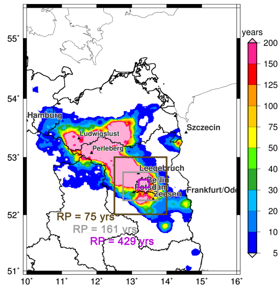
Figure 10. Return periods of the 24 h precipitation totals based on REGNIE using a Gumbel distribution (extreme value type 1; reference period: 1951–2020). Note: all return periods above 200 years are shown uniformly in one colour due to statistical uncertainty (see text for more information). Coloured polygons (in pink, grey, brown) including the associated averaged return periods (RP) indicate three different-sized averaging areas explained in Table S2 and in the text.
