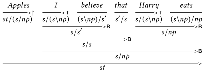
Figure 8.12: Analysis of long-distance dependencies across sentence boundaries
