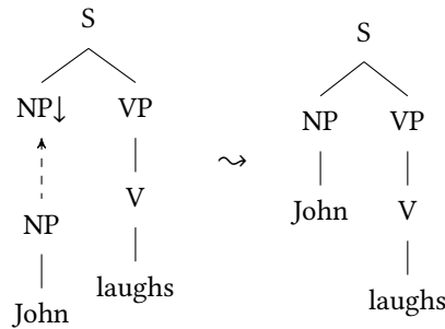
Figure 12.2: Substitution
