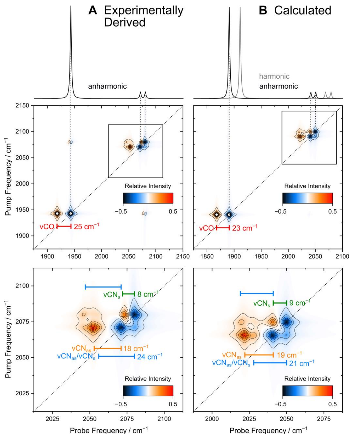
Figure 3. Linear IR absorption spectra ( top ) and absorptive 2D-IR spectra ( center and bottom ) of the \text{Ni}_a\text{-S} state of [\text{NiFe}] hydrogenase, simulated from (A) experimental and (B) calculated transition frequencies. Signals in harmonic ( grey ) and anharmonic ( black ) absorption spectra are represented as Lorentzian lines. Two-dimensional-IR spectra are shown as contour plots for the entire \nu\text{CX} spectral region ( center ) and the region characteristic for \nu\text{CN} vibrations ( bottom ). These spectra were obtained by two-dimensional Fourier transform of the third-order response for \langle\text{ZZZZ}\rangle polarisation, as detailed in the Materials and Methods section. Since the simulation of the 2D-IR spectra employs the harmonic approximation for scaling intensities of excited-state transitions, spectra throughout the entire figure are based on harmonic transition dipole strengths. In case of the 2D-IR contour plots, transition dipole strengths of \nu\text{CN} fundamental transitions were multiplied by a factor of 10 for better cognition. Relevant intra- and intermode anharmonicities, \Delta\omega_{1-2}^a and \Delta\omega_{a/b} , are indicated for \nu\text{CO} and \nu\text{CN} vibrations.
