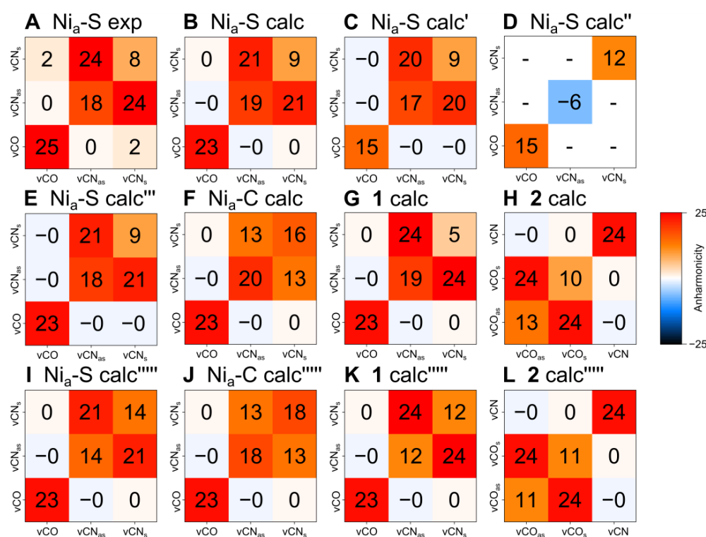
Figure 4. Matrix representation of intramode anharmonicities \Delta\omega_{1-2}^a and intermode anharmonicities \Delta\omega_{a/b} of \nu\text{CX} ligand stretch vibrations. Diagonal entries correspond to \Delta\omega_{1-2}^a , while off-diagonal entries correspond to \Delta\omega_{a/b} . (A) Ni a -S state of [NiFe] hydrogenase, experiment. (B) Ni a -S state of [NiFe] hydrogenase, calculated. All vibrational degrees of freedom were included in the anharmonic analysis. (C) Ni a -S state of [NiFe] hydrogenase, calculated. Only interacting \nu\text{CO} and \nu\text{CN} vibrations were included in the anharmonic analysis ( \Delta\omega_{1-2}^{\nu\text{CO}'} and \Delta\omega_{a/b}' ). (D) Ni a -S state of [NiFe] hydrogenase, calculated. Only non-interacting \nu\text{CO} and \nu\text{CN} vibrations were included in the anharmonic analysis ( \Delta\omega_{1-2}^{\nu\text{CO}''} ). (E) Ni a -S state of [NiFe] hydrogenase, calculated. Only interacting \nu\text{CO} , \nu\text{CN} , \nu\text{Fe-CO/CN} , and \delta\text{Fe-CO/CN} vibrations were included in the anharmonic analysis ( \Delta\omega_{1-2}^{\nu\text{CO}''''} and \Delta\omega_{a/b}'''' ). (F) Ni a -C state of [NiFe] hydrogenase, calculated. All vibrational degrees of freedom were included in the anharmonic analysis. (G) Model complex 1, calculated. All vibrational degrees of freedom were included in the anharmonic analysis. (H) Model complex 2, calculated. All vibrational degrees of freedom were included in the anharmonic analysis. (I) Ni a -S state of [NiFe] hydrogenase, calculated. All vibrational degrees of freedom were included in the anharmonic analysis, but 2-2 Darling-Dennison (DD) resonances were not considered ( \Delta\omega_{1-2}^{\nu\text{CO}''''} and \Delta\omega_{a/b}'''' ). (J) Ni a -C state of [NiFe] hydrogenase, calculated. All vibrational degrees of freedom were included in the anharmonic analysis, but 2-2 DD resonances were not considered. (K) Model complex 1, calculated. All vibrational degrees of freedom were included in the anharmonic analysis, but 2-2 DD resonances were not considered. (L) Model complex 2, calculated. All vibrational degrees of freedom were included in the anharmonic analysis, but 2-2 DD resonances were not considered. \delta —bending vibration; \nu —stretching vibration.
