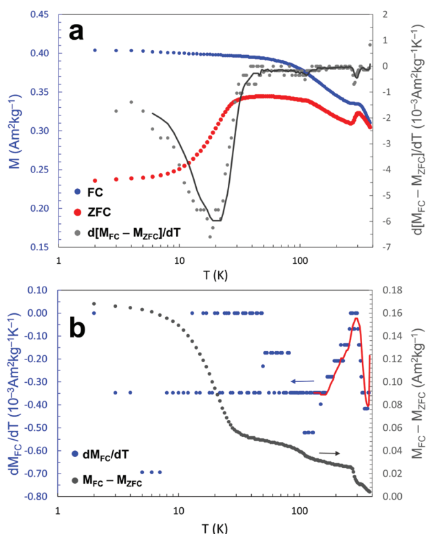
Figure 2. Temperature-dependent magnetization curves. a) Left axis: FC and ZFC curves under an applied field of 5 mT. Blue: FC, Red: ZFC. Right axis: d[M_{FC} - M_{ZFC}]/dT as a function of increasing temperature. Gray dots: calculated values, Gray line: fitted trendline. The minimum at around 20 K indicates the freezing temperature of the spin-glass phase. b) Left axis: dM_{FC}/dT as a function of the temperature. Blue: calculated values, Red: fitted trendline. The local maximum at around 314 K indicates the Néel temperature of the AFM phase. Right axis M_{FC} - M_{ZFC} variation as a function of the temperature (gray dots). The extrapolated intercept with the x-axis shows that the bifurcation temperature (irreversibility) is higher than the accessible experimental temperature range ( >380 K).
