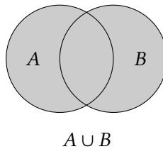
Figure 13.3: Set union
