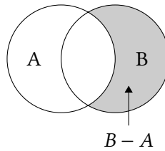
Figure 13.4: Set complementation
