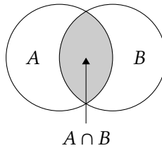
Figure 13.2: Set intersection
