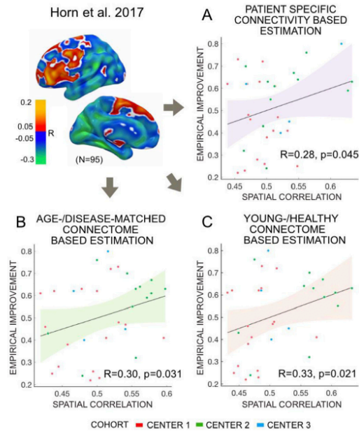
Fig. 4. Validation of optimal connectivity profiles estimated in, Hom et al., 2017b ) on the present three-center cohort ( N = 33 ), in which individual dMRI data was available. Clinical improvements could be significantly estimated using patient-specific connectivity (A), a disease-/age-matched connectome (B) and a young-/healthy connectome (C).
