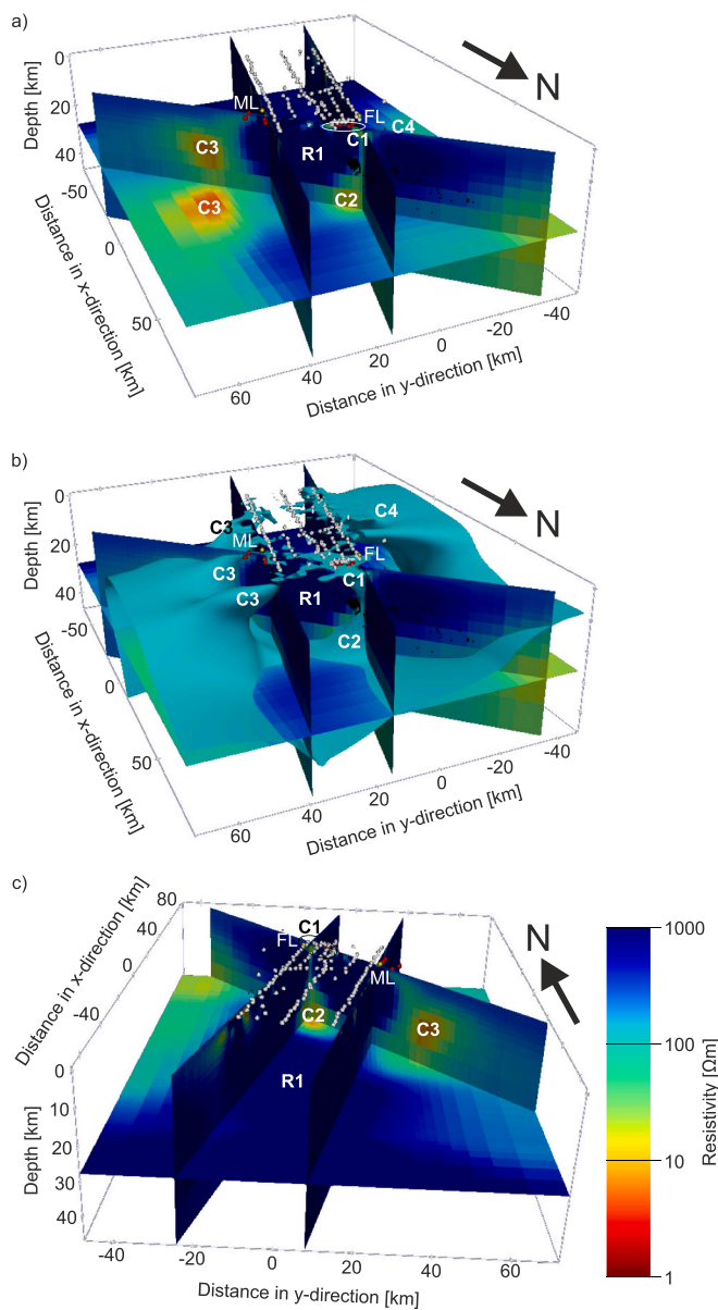
Fig. 9. Pseudo-sections showing the most important structures from different directions. The depth slice corresponds to a depth of 27.6 km. a) The most prominent conductors C2 and C3 form reservoirs at larger depths and continue in form of conductive channels from the reservoir up to the surface where they seem to correlate with location of mofettes (red dots) close to FL and ML. b) Same pseudo-sections as in a) overlain by a 150 \Omega\text{m} isosurface visualizing the different conductive branches of C3 and the shape of the conductor C4 in the southwest. c) Large parts of the study area, especially in the south, are dominated by high resistivities possibly related to the crystalline basement. (For interpretation of the references to colour in this figure legend, the reader is referred to the web version of this article.)
