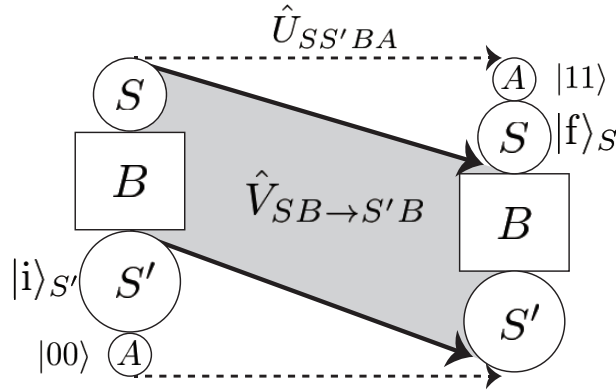
FIG. 1. A schematic of a generalized thermal operation (Definition 3). The partial isometry \hat{V}_{SB \rightarrow S'B} can be embedded into the energy-conserving unitary \hat{U}_{SS'BA} of the composite system SS'B along with a 2-qubit auxiliary system A . The initial state of S'A is chosen as a pure state |i\rangle_{S'}|00\rangle and the final state of SA is projected onto |f\rangle_S|11\rangle . Here, |i\rangle_{S'} and |f\rangle_S can be arbitrary energy eigenstates of S' and S , and the Hamiltonian of A is chosen as a function of these energies to ensure the global energy conservation.
