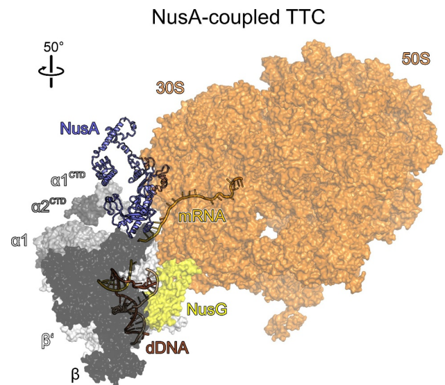
Figure 5. Semi-transparent surface representation of a NusA-coupled TTC (PDB ID 6X7F). Ribosome subunits are shown in Orange. NusA act as a “coupling-pantograph” between RNAP and the 30S ribosomal subunit. NusA is constantly but flexibly linked to RNAP via its NTD and AR2 domains, providing NusA with a high degree of conformational freedom between RNAP and the 530 subunit, which could facilitate NusA to make favorable contacts to the nascent RNA transcript.
