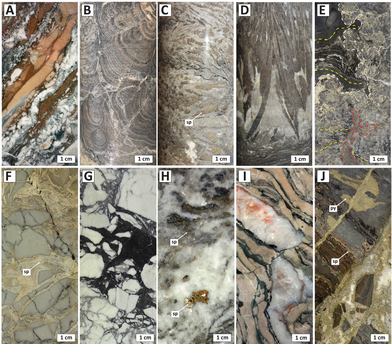
Fig. 9. Hand sample photographs of HTD and vein assemblages. A. Partial secondary dolomite ( \pm quartz) replacement of nodular dolostone beds in the W-Fold Shale Member (TNDD015 @ 772 m). B. Botryoidal HTD (TNDD033 @ 1,025.5 m). C. Sideways radiating bladed dolomite with interstitial sphalerite and quartz (TNDD014 @ 705 m). D. Downward radiating fan of coarse HTD blades (after aragonite) with interstitial dolomite (TNDD017 @ 903.4 m). E. Massive HTD replacement with interstitial sphalerite and pyrite mineralization overprinting laminated pyritic carbonaceous shale from middle W-Fold Shale Member. Yellow dashed line shows relic bedding traces (TNDD11A @ 1,118 m). F. Sphalerite-cemented hydrothermal breccia (poststylobreccia) in Teena Dolostone from Jabiru fault zone (Teena4 @ 800 m). G. Black-matrix dolomite jigsaw to rubble breccia in Teena Dolostone (poststylolite; TNDD008 @ 639 m). H. Stockwork ankerite veining overprinting HTD (TNDD015 @ 831 m). I. Late-stage bedding-parallel quartz vein with trace hematite in W-Fold Shale Member (TNDD014 @ 1,104 m). J. High-angle late-stage quartz-carbonate-pyrite veins cutting mineralized Lower HYC unit (TNDD014).
