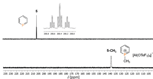
Fig. 2 ^{31}\text{P} NMR of 5 (25 °C) and 5-CH 3 ( T = -70 °C) in \text{CD}_2\text{Cl}_2 .
