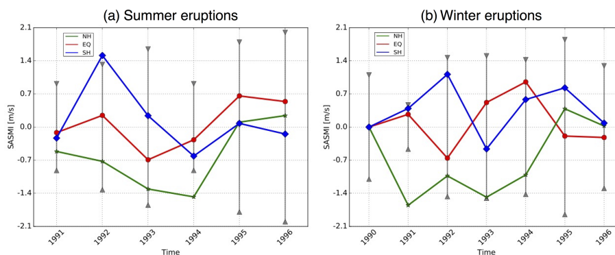
Figure 7. South Asian summer monsoon index ( \text{m s}^{-1} ) anomaly for the summer eruption cases (a) and the winter eruption cases (b). The grey bar indicates 1 standard deviation of the control runs.
