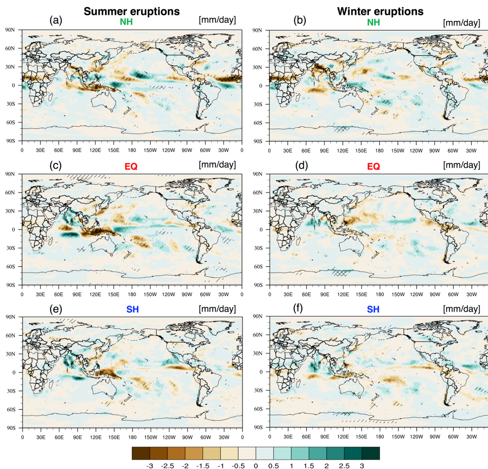
Figure 5. Spatial distribution of JJA mean precipitation ( \text{mm d}^{-1} ) anomaly in 1992 for the summer NH (a), EQ (c) and SH (e) eruption cases and in 1991 for the winter NH (b), EQ (d) and SH (f) eruption cases. The cross signs and slashes indicate the grid points with significant differences based on the two-tailed Student's t tests at the 95 % and 99 % confidence level, respectively.
