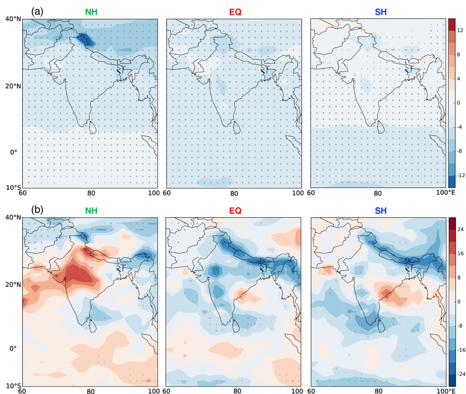
Figure 9. Spatial distribution of JJA mean net surface solar radiation ( \text{kg m}^{-2} ) anomaly in clear-sky (a) and all-sky conditions (b) after the NH (left), EQ (middle) and SH (right) volcanic eruptions in 1992. The vertical bars and plus signs indicate the grid points with significant differences based on the two-tailed Student's t test at the 95 % and 99 % confidence level, respectively.
