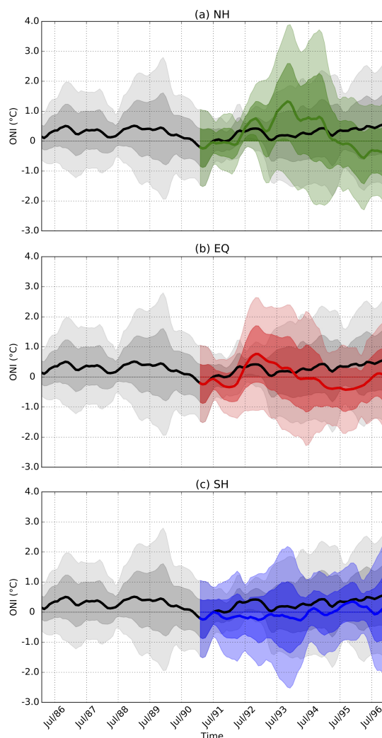
Figure 12. Time series of Oceanic Niño Index ( ^{\circ}\text{C} ) anomaly for the NH (a), EQ (b) and SH (c) volcanic eruption cases. The black and relative solid color lines are the ensemble member means of the control run and the eruption cases. The dark and light grey and relative heavy and light color shades represent 1 and 2 standard deviation of the control runs and the eruption cases.
