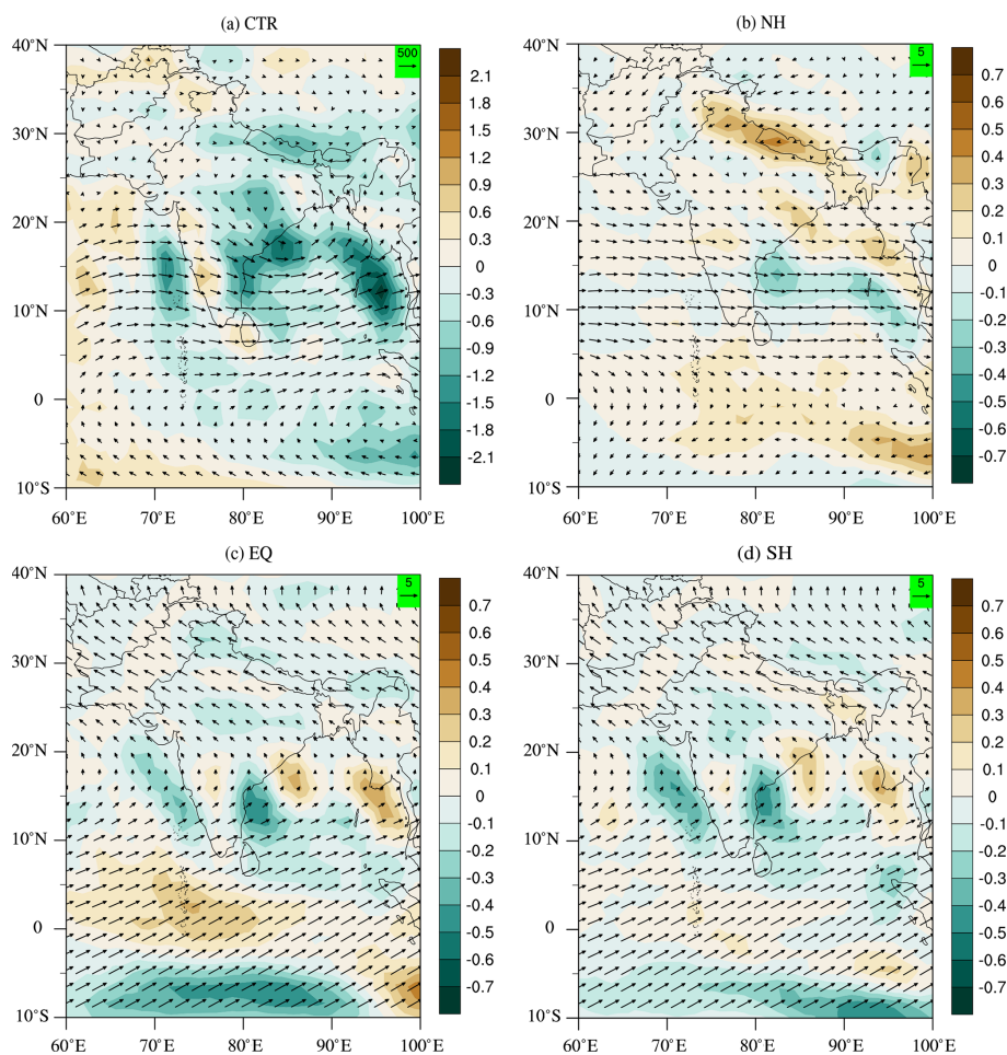
Figure 8. JJA mean vertically integrated moisture transport (IVT, vector, \text{kg m}^{-1} \text{s}^{-1} ) and its divergence (IVTD, shaded, \text{kg m}^{-2} \text{s}^{-1} ) for the control runs without any volcanic eruption (a), and their anomalies after the NH (b), EQ (c) and SH (d) volcanic eruptions in 1992.
