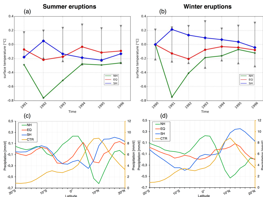
Figure 6. Difference of JJA mean temperature ( ^{\circ}\text{C} ) anomaly between the Northern and the Southern Hemisphere after the summer eruptions (a) and the winter eruptions (b), and the position of the ITCZ in 1992 (c) and 1991 (d) indicated by the JJA mean zonal mean precipitation ( \text{mm d}^{-1} ) anomaly between 20^{\circ}\text{N} and 20^{\circ}\text{S} . The yellow line (right axis) in (c) and (d) indicates the position of the ITCZ for the control runs, which is calculated with raw precipitation data. The grey bar in (a) and (b) indicates the 2 standard deviation of the control runs.
