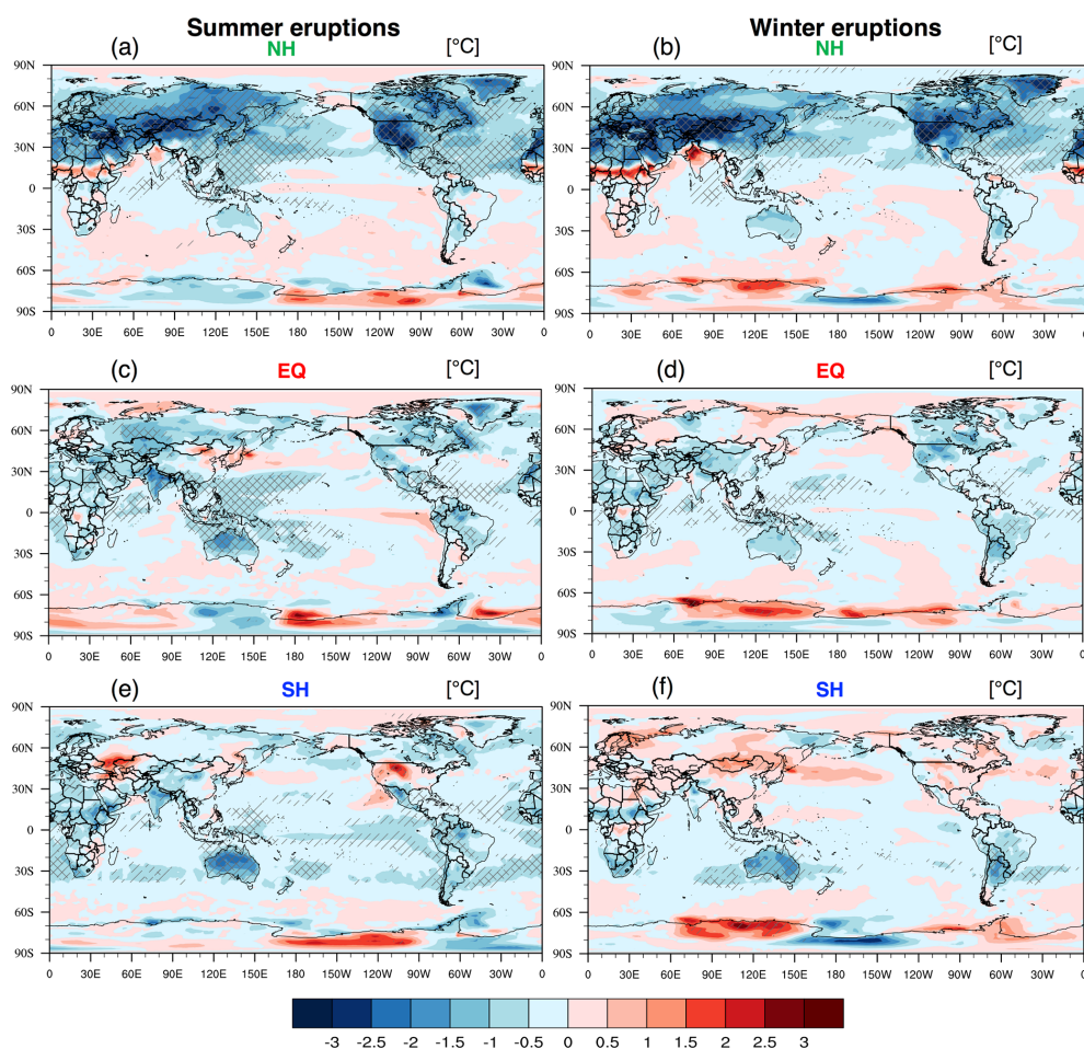
Figure 4. Spatial distribution of JJA mean temperature ( ^{\circ}\text{C} ) anomaly in 1992 for the summer NH (a), EQ (c) and SH (e) eruption cases and in 1991 for the winter NH (b), EQ (d) and SH (f) eruptions cases. The cross signs and slashes indicate the grid points with significant differences based on the two-tailed Student's t test at the 95 % and 99 % confidence level, respectively.
