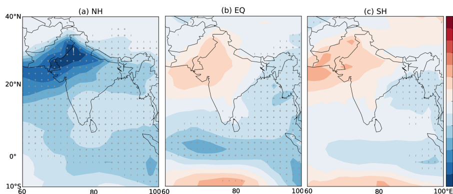
Figure 11. Spatial distribution of JJA mean vertical integrated water vapor ( \text{kg m}^{-2} ) anomaly after the NH (a), EQ (b) and SH (c) summer volcanic eruptions in 1992. The vertical bars and plus signs indicate the grid points with significant differences based on two-tailed Student's t tests at the 95 % and 99 % confidence level, respectively.
