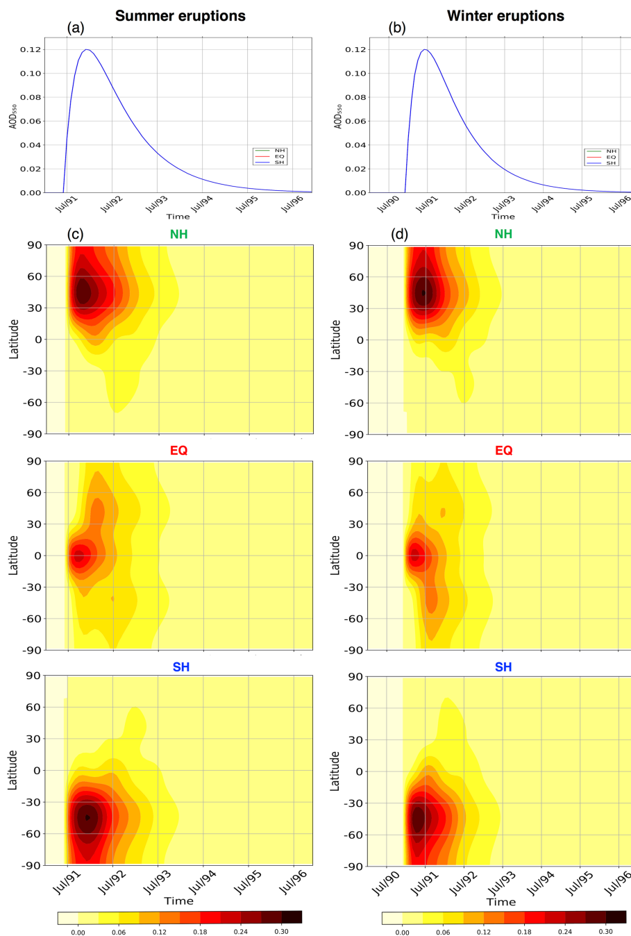
Figure 1. Global mean aerosol optical depth anomaly at 550 nm for the summer (a) and winter (b) volcanic eruption cases and their zonal mean distributions (c, d).
