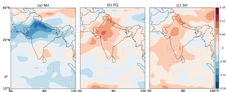
Figure 10. Spatial distribution of JJA mean total cloud cover (%) anomaly after the NH (a), EQ (b) and SH (c) volcanic eruptions in 1992. The vertical bars and plus signs indicate the grid points with significant differences based on the two-tailed Student's t tests at the 95 % and 99 % confidence level, respectively.
