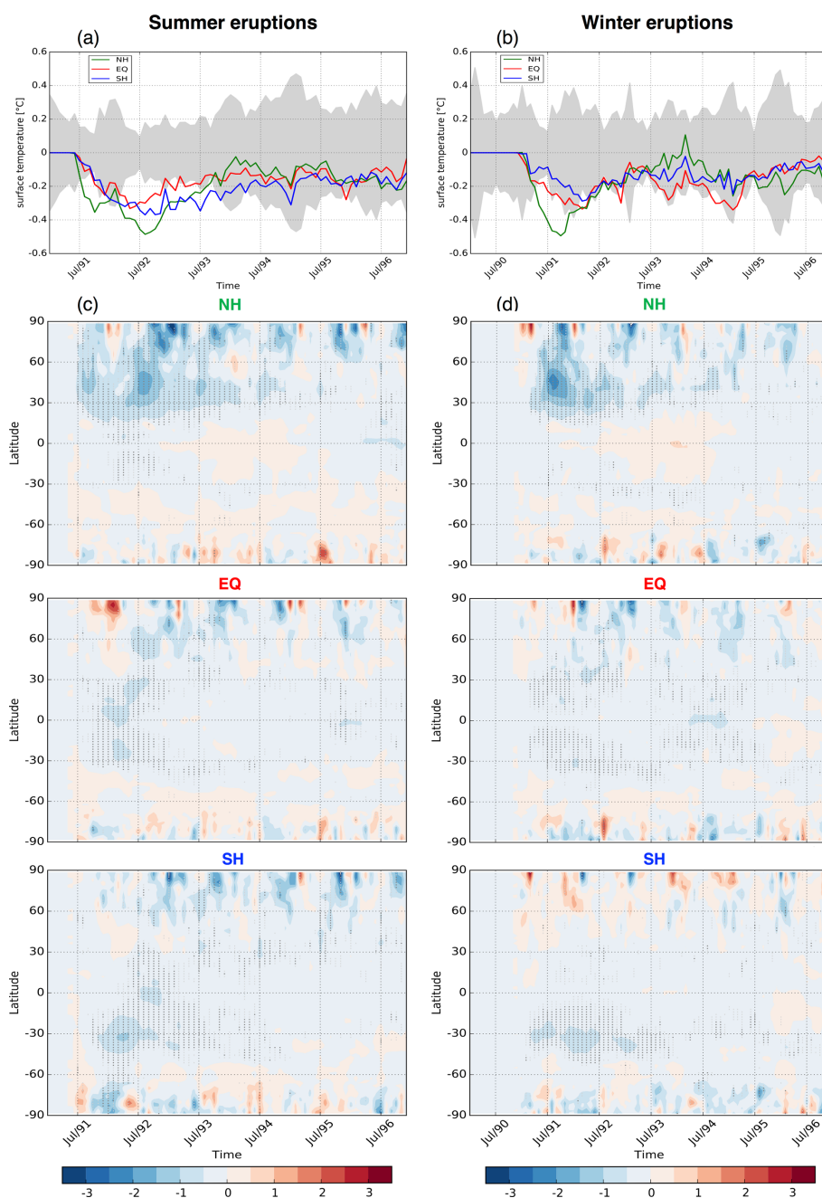
Figure 3. Global mean surface temperature ( ^{\circ}\text{C} ) anomaly for the summer (a) and winter (b) volcanic eruption cases and their zonal mean distributions (c, d). The grey shading in (a) and (b) indicates 2 standard deviations around the mean of the control runs without any volcanic eruption. Dark grey and light grey stippling in (c) and (d) indicate the grid points with significant differences based on the two-tailed Student's t test at the 95 % and 99 % confidence level, respectively.
