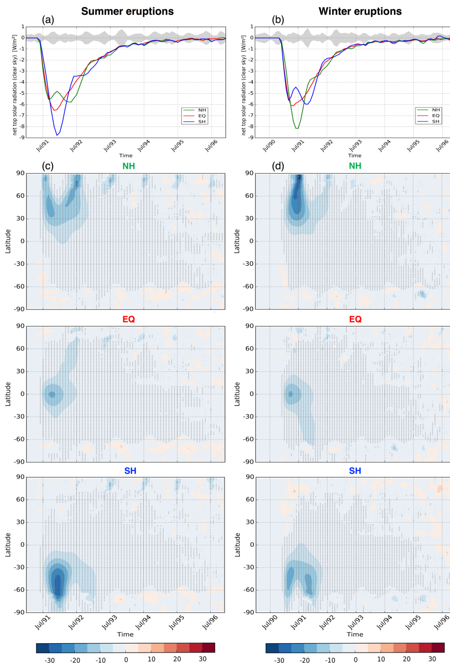
Figure 2. Global mean net outgoing solar radiation ( \text{W m}^{-2} ) anomaly at the top of the atmosphere in clear-sky conditions for the summer (a) and winter (b) volcanic eruption cases and their zonal mean distributions (c, d). The grey shading in (a) and (b) indicates 2 standard deviation of the control runs without any volcanic eruption. Dark grey and light grey stippling in (c) and (d) indicate the grid points with significant differences based on the two-tailed Student's t test at the 95 % and 99 % confidence level, respectively.
