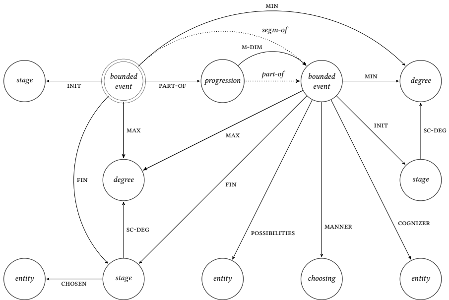
Figure 1.1: Graph representation of the verb dovybirat 2PF 'to finish electing'
