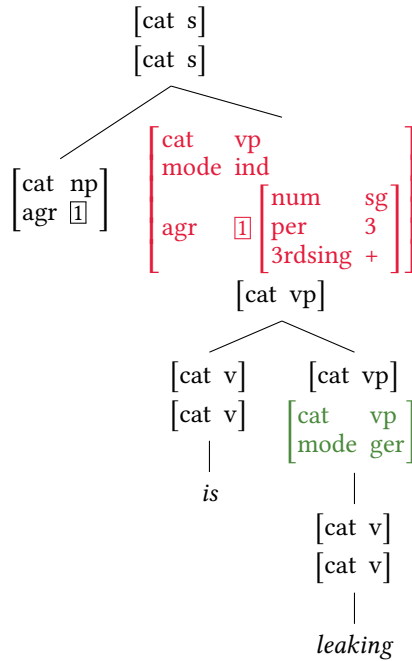
Figure 6.5: Adjunction of is into the tree for leaking : result
