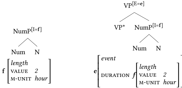
Figure A.12: Frame representation of the time adverbial 2 časa ‘for 2 hours’ before and after enriching its structure
