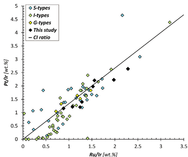
Fig. 10. Compositional data from PGNs exposed at the surfaces of six S-types and one G-type cosmic spherule derived from the Meppen micrometeorite collection (note that although we identified nine particles with PGNs, two lacked detectable Ir). The Meppen PGNs are compared against previously reported PGNs found in micrometeorites (S-, I-, and G-types). Data were taken from Brownlee et al. (1984), Bonté et al. (1987), and Rudraswami et al. (2011, 2014), while CI data were calculated from Tagle and Berlin (2008). All data are plotted as elemental ratios (calculated from their raw wt% data). We selected ratios since these are significantly more accurate than absolute abundance data. The PGN compositions of the Meppen particles were determined by standardless EDS on their topographically complex surfaces (raw data shown in Table 2). In contrast, literature data also used EDS but predominantly obtained from the polished flat surfaces of micrometeorite interiors. This plot demonstrates that the PGNs in micrometeorites (including those recovered from the Meppen rooftop) have chondritic elemental abundance for PGE elements. Furthermore, the similarity between PGN compositions in S-, I-, and G-type particles supports the conclusion that they all form in the same way from a chondritic source, concentrated by the oxidation of chondritic materials. (Color figure can be viewed at wileyonlinelibrary.com .)
