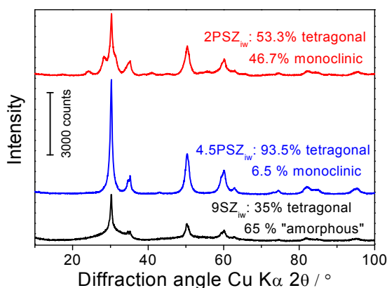
Figure 7-4: X-ray diffractograms of calcined 2PSZ iw , 4.5PSZ iw and 9SZ iw .
