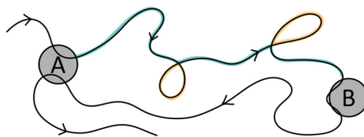
Fig. 7 Splitting of a reactive trajectory into one productive path from A to B (in blue) and several unproductive cycles (yellow)
