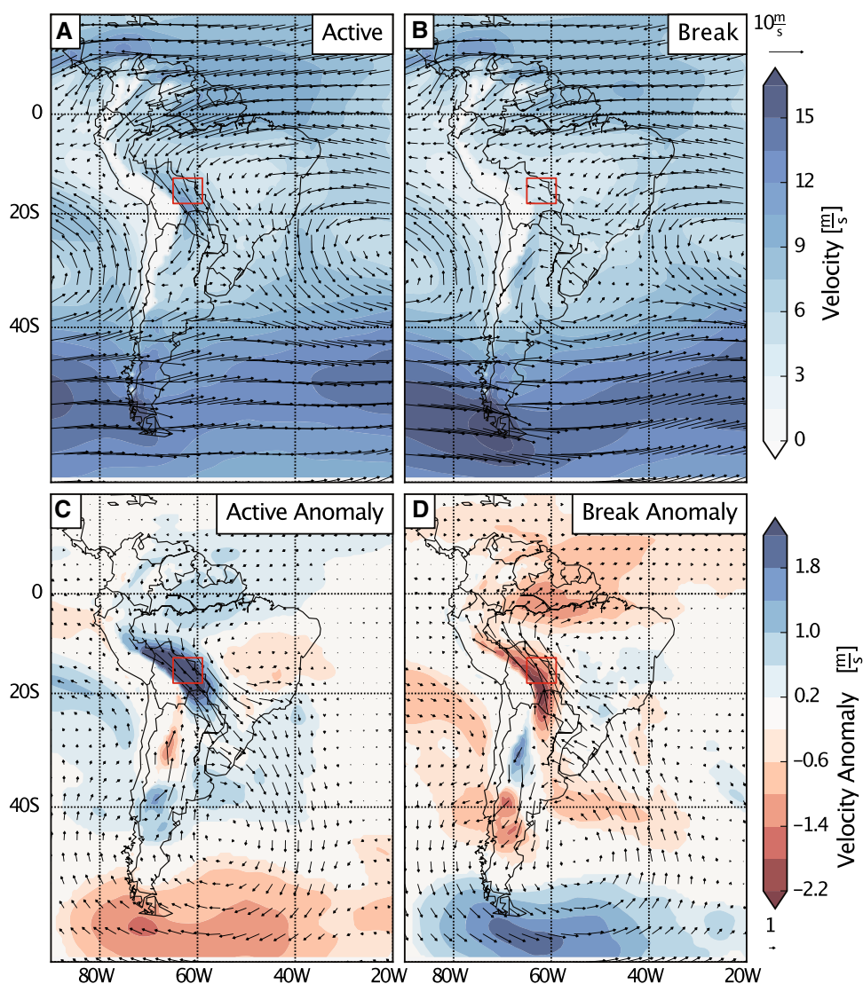
Fig. 4 Wind fields at 850 hPa during active (westerly, A and C ) and break (easterly, B and D ) regimes for the DJF season. The arrows indicate the wind direction and strength. The top row ( A , B ) uses the regular meridional and zonal wind components during the active and break phases, respectively. The bottom row C , D shows anomalous wind fields, which were computed by removing the seasonal mean componentwise from the wind vector. The absolute value of the wind is color-coded in all subfigures. The bottom row panels show the anomalous absolute value, which was computed by removing the mean from the absolute value and performing a one-sample t-test. Only absolute value anomalies at a 95% significance level are shown. During the active phase the South American Low-Level Jet (SALLJ) is visibly enhanced. Between the active and the break phases the direction of the anomalous wind vectors is reversed
