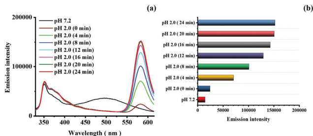
Fig. 5 (a) Emission spectra and (b) bar graph of the response time of the fluorescence of dyad 8 observed upon addition of dyad 8 to a THF–H 2 O mixture (1 : 1) in B–R buffer (25 mM) of pH 2.0; excitation \lambda_{\text{Ex}} was at 315 nm and the fluorescence intensity was recorded at an emission wavelength \lambda_{\text{em}} of 582 nm. The emission spectra of dyad 8 were recorded every 4 min. The data obtained at pH 7.2, where no ring opening should occur, are included as control.
