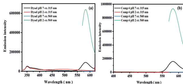
Fig. 6 Emission spectra recorded at excitation wavelength of 315 nm and 560 nm at pH 7.0 and 2.0 (3.3 \mu\text{M} ) of (a) dyad 8 and (b) compound 6 in a THF–H 2 O mixture (1 : 1) in B–R buffer (25 mM).
