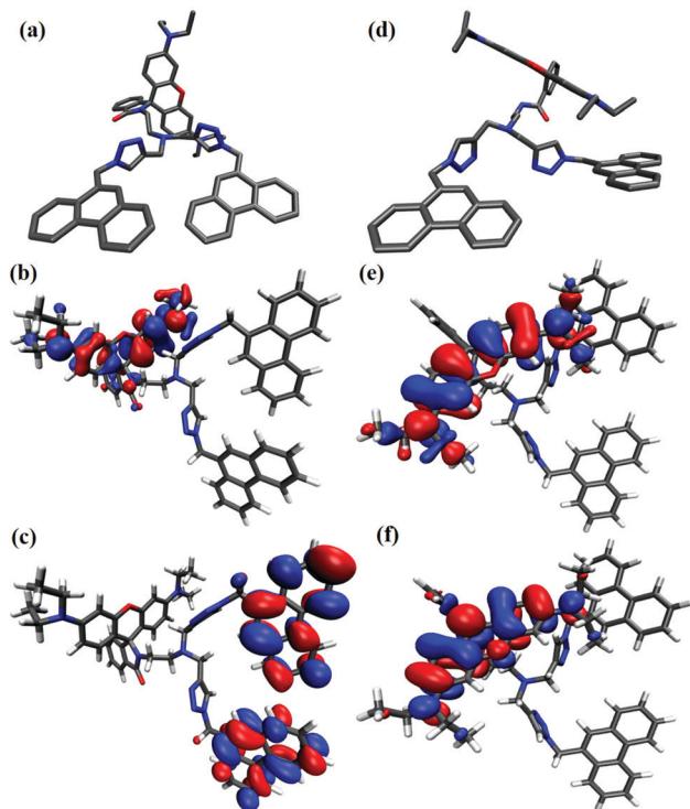
Fig. 8 DFT optimized structures of dyad 8 (a) and its \mathbf{8} + \text{H}^+ ; protonated form (d); HOMO (b) and LUMO (c) isosurfaces of dyad 8 and protonated form HOMO (e) and LUMO (f) obtained at the \omega\text{B97X-D3/def2-TZVP} level. Plots were generated using ORBKIT, isovalue = 0.02a_0^{-3.54-57}
