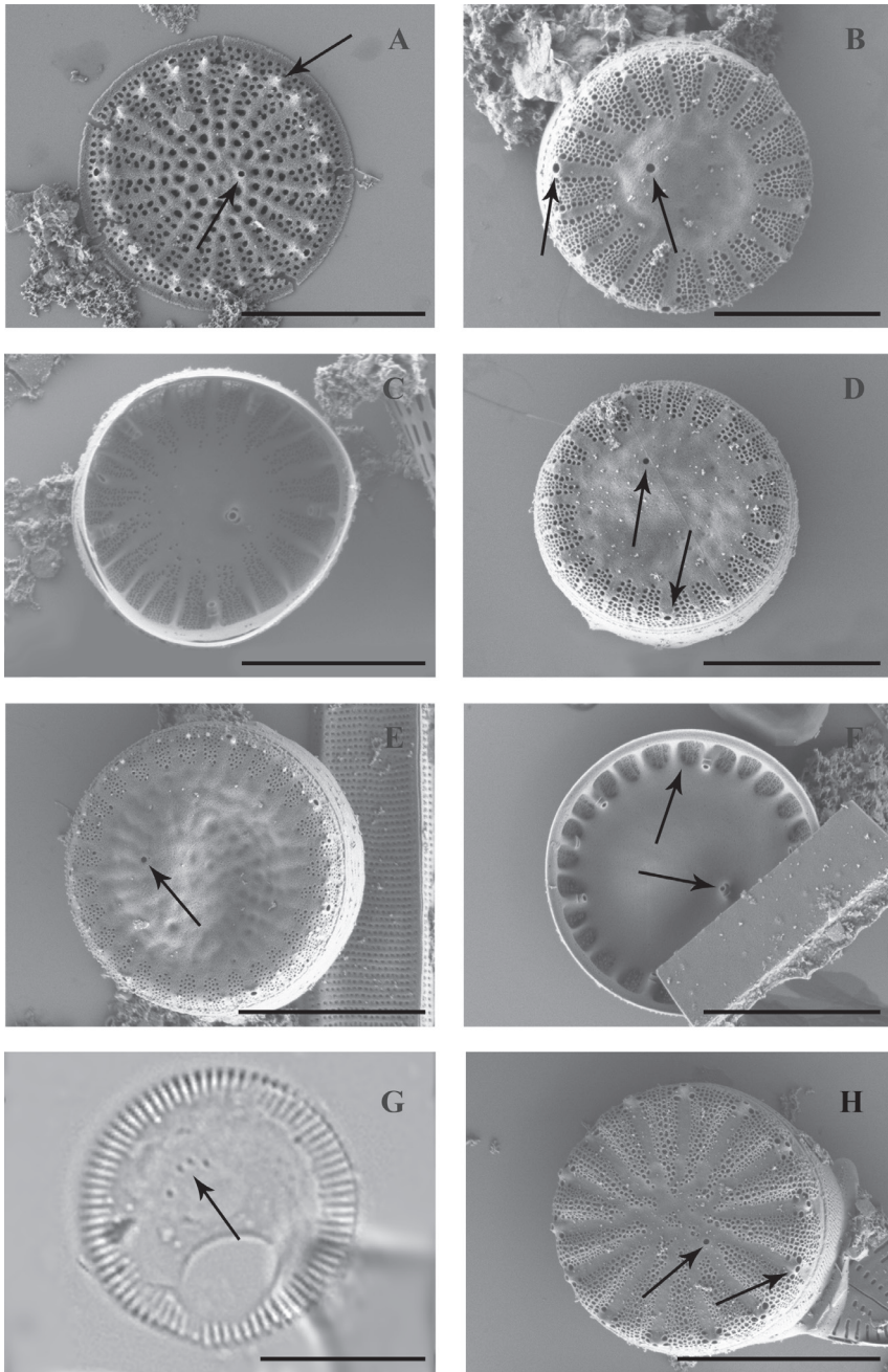
Figure 6. SEM (A–F, H) and LM images (G) of species found in the transitional zone at Mykolaiv city, valve views: A Stephanodiscus minutulus with arrows shown marginal and central fultoportulae B, C Cyclotella atomus var. atomus with arrows shown marginal and central fultoportulae D–F Cyclotella atomus var. gracilis with arrows shown marginal and central fultoportulae on D picture, only central fultoportula on E and central fultoportula and alveolae on (F) G Cyclotella choctawhatcheeana with arrow shown central fultoportulae H Cyclotella cryptica with arrows shown marginal and central fultoportulae. Scale bars: 3 \mu\text{m} (B, C); 4 \mu\text{m} (D, F); 5 \mu\text{m} (A, E, H); 10 \mu\text{m} (G).
