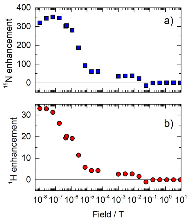
Figure 8. Field dependence of 15 N NMR signals (a) and 1 H NMR signals (b) corresponding to singlet order of the 15 N spin pair in cis - 15 N 2 -ABZ hyperpolarized by SABRE SHEATH. The experimental protocol for the SABRE experiments is shown in Figure 2b. All the functions were normalized by the integral intensity of the corresponding signal intensity at thermal equilibrium.
