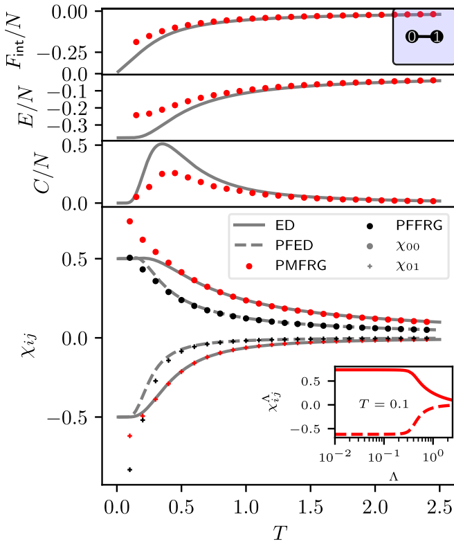
FIG. 3. (Free) energy, heat capacity per spin, and static susceptibilities of the Heisenberg dimer with J = 1 obtained via PMFRG (red symbols) at \Lambda = 0 as a function of temperature. Displayed in solid (dashed) gray lines are the results obtained by (pseudofermion) exact diagonalization, as well as the finite-temperature spin susceptibilities of the PFFRG in black symbols. Each data point corresponds to a fully converged flow with respect to \Lambda as demonstrated in the exemplary plot at T = 0.1 (cf. Fig. 2).
