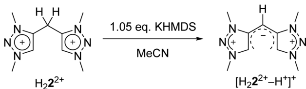
Scheme 3 Synthesis of [\text{H}_2^{2+}-\text{H}^+]^+ .
