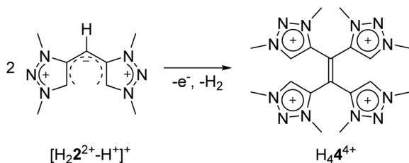
Scheme 4 Formation of \text{H}_4^{4+} from [\text{H}_2^{2+}-\text{H}^+]^+ .
