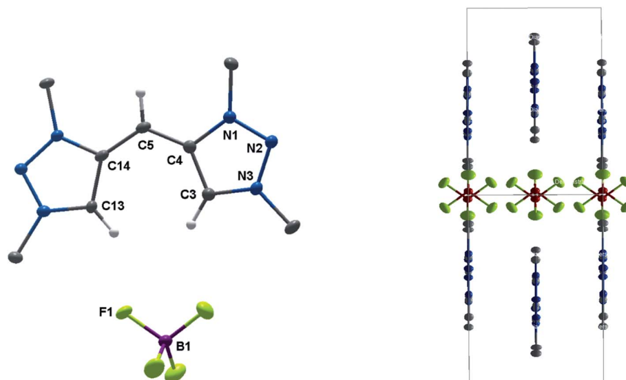
Fig. 9 ORTEP representation of [\text{H}_2\text{2}^{2+}-\text{H}^+](\text{BF}_4) : ellipsoids drawn at 50% probability. H-atoms (except those at C3, C5 and C13) are omitted for clarity. (Left) Single molecule, (right) unit cell (for selected bond length and angles see ESI Table S4 † ).
