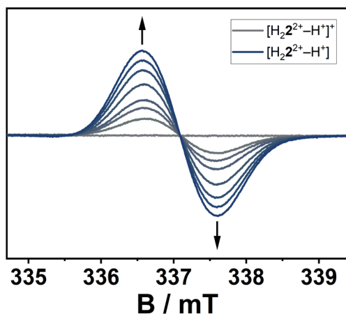
Fig. 10 EPR-spectroelectrochemical measurement of [\text{H}_2^{2+}-\text{H}^+]^+ with 0.1 M \text{NBu}_4\text{PF}_6 in acetonitrile, electrolysis at 0.8 V versus silver wire at 0 °C.
