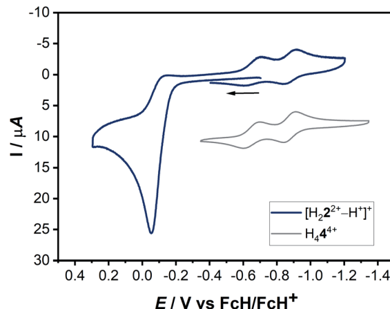
Fig. 11 Combined cyclic voltammograms of a 0.1 mM solution of [\text{H}_2^{2+}-\text{H}^+]^+ and \text{H}_4^{4+} with 0.1 M \text{NBu}_4\text{PF}_6 in acetonitrile at 100 \text{mV s}^{-1} .
