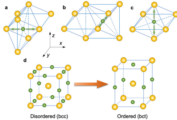
Fig. 1 | Disorder-order transition in Fe-C alloys. a-c, C occupation on three octahedral sublattices and its induced tetragonal deformation (green arrows). Large orange spheres denote Fe atoms and small green spheres refer to C atoms. d, Schematic illustration of the disorder-order transition. Green spheres show the possible sites for C to randomly occupy in a unit cell, but they are not all occupied.
