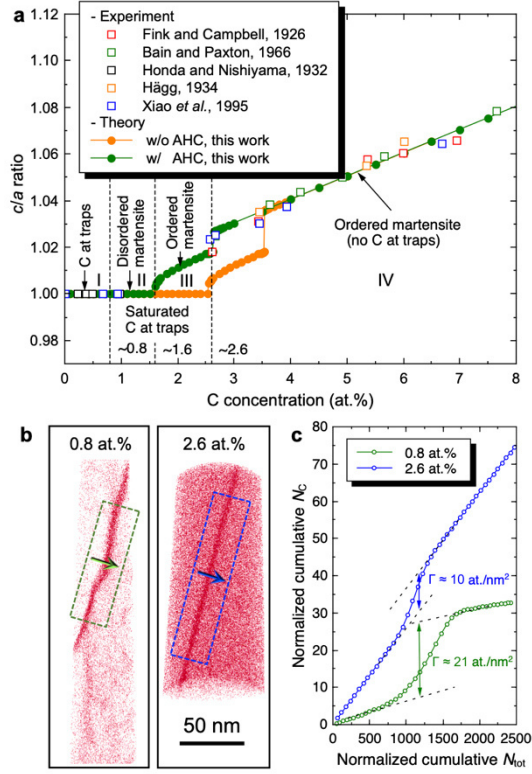
Fig. 5 | Comparison between theory and experiment. a , Comparison of experimental and theoretically computed c/a ratio of Fe-C alloys as a function of C concentration at room temperature. The experimental data are collected from refs. [33–37]. b , APT analysis of the C distribution in two representative alloy samples with 0.8 and 2.6 at.% C. The regions highlighted by the green ( 30 \times 26 \times 94 nm 3 ) and blue ( 30 \times 37 \times 131 nm 3 ) rectangles along the grain boundaries are selected for a quantitative analysis of C excess. c , Gibbsian interfacial excess of C for the two alloy samples. N_c and N_{tot} are the cumulative number of C and of all atoms, respectively, normalized by the selected grain boundary areas.
