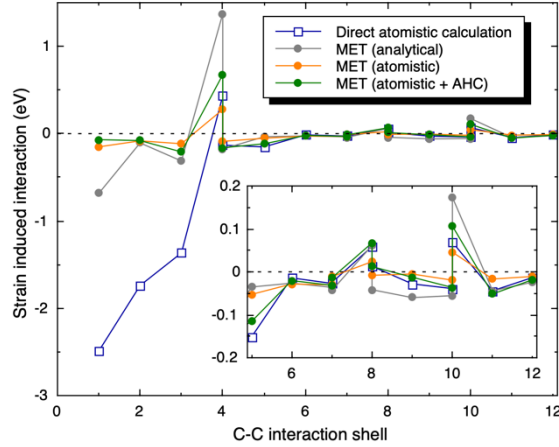
Fig. 2 | Strain induced interaction. Strain induced interaction between two C interstitials in bcc Fe from different approaches. The inset provides an enlarged view for the interactions at the 5 th –12 th shells. “AHC” stands for anharmonic contribution.
