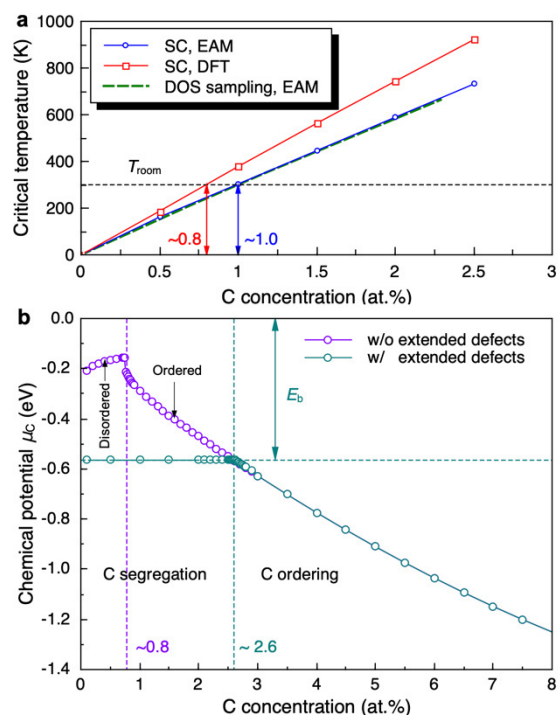
Fig. 4 | Competition between C ordering and segregation. a , Calculated critical temperature as a function of C concentration using the self-consistent defect-chemistry (“SC”) approach with EAM or DFT input compared to the result obtained from the DOS sampling approach. b , Chemical potential of C ( \mu_C ) at room temperature as a function
