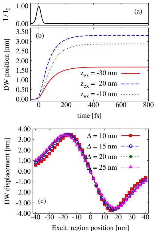
FIG. 5. (Color online) Laser-induced dynamics of the domain wall. (a) Time variation of Gaussian laser pulse intensity with peak at time t = 0 and FWHM 35 fs. (b) Time dependence of the domain wall position after the laser pulse for DW width \Delta = 10 nm calculated for different positions of the excitation region. (c) DW displacement taken 1 ps after the DW motion for different DW widths as a function of the excitation region position.
