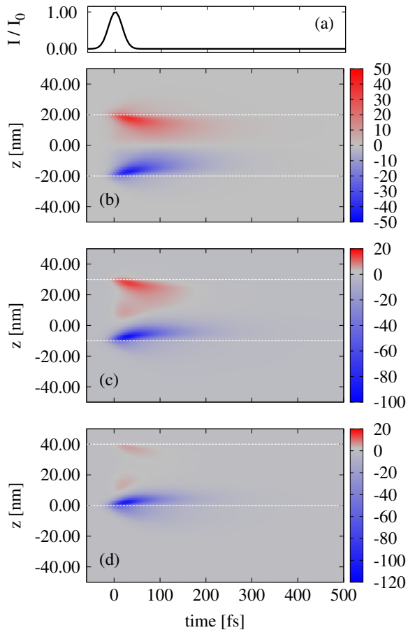
FIG. 4. (Color online) Spatial and time dependence of the transverse spin current in the neighborhood of a domain wall in the units of [\hbar/(2e)] \text{ fs}^{-1} . The domain wall center is located in z = 0 and its width is \Delta = 10 \text{ nm} . The excitation region is restricted to the area between the white dashed lines. (a) Time variation of Gaussian laser pulse intensity with peak at time t = 0 and FWHM 35 fs. (b) The excitation region is symmetric with respect to the position of the domain wall center. (c) and (d) The excitation region is asymmetric with respect to the position of the domain wall center. In case (d) the borderline of the excitation region passes through the domain wall center.
