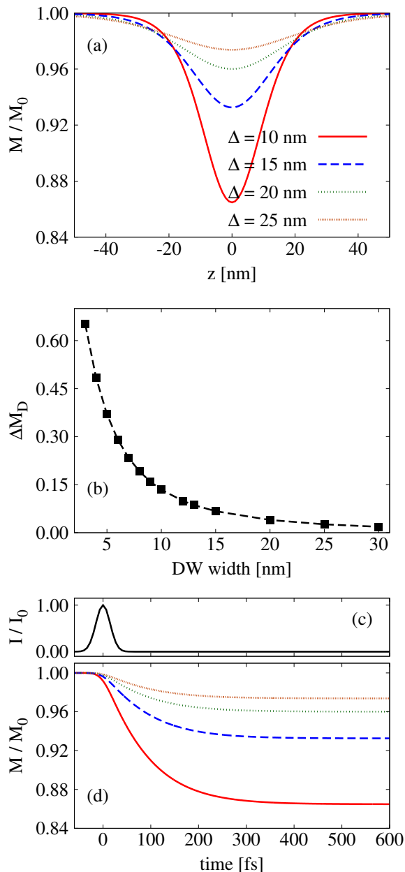
FIG. 3. (Color online) Laser-induced demagnetization in the vicinity of the domain wall calculated for various DW widths. (a) Spatial dependence of magnetization taken 1 ps after the pulse. (b) Demagnetization in the DW center, z = 0 , taken 1 ps after the pulse as a function of the DW width. (c) Time variation of Gaussian laser pulse intensity with peak at time t = 0 and FWHM 35 fs. (d) Time-dependence of magnetization in the DW center after the laser pulse, for various DW widths. The lines correspond to those shown in (a).
