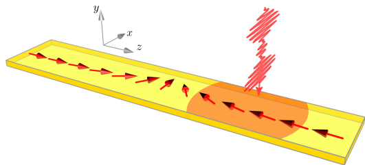
FIG. 1. (Color online) Sketch of a head-to-head magnetic domain wall and the used coordination system. The wavevector of the incident laser beam is aligned with the y axis.
