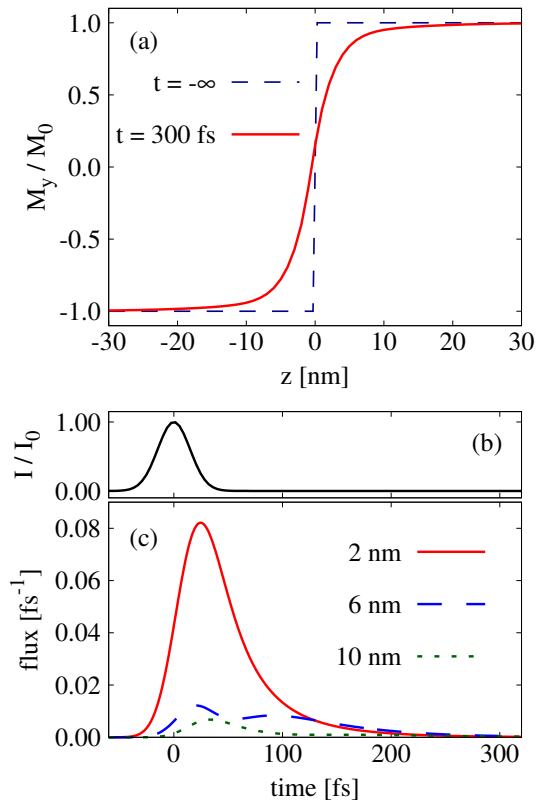
FIG. 2. (Color online) Superdiffusive transport through a narrow magnetic domain wall. (a) Dashed (blue) line shows out-of-plane component of magnetization in the vicinity of a narrow magnetic domain wall in the equilibrium ( t = -\infty ). Solid (red) line shows the out-of-plane magnetic component 300 fs after the maximum of the laser pulse. (b) Time variation of Gaussian laser pulse intensity with peak at time t = 0 and FWHM 35 fs. (c) Corresponding time variation of the spin fluxes calculated for different distances (2, 6, and 10 nm) from the domain wall.
