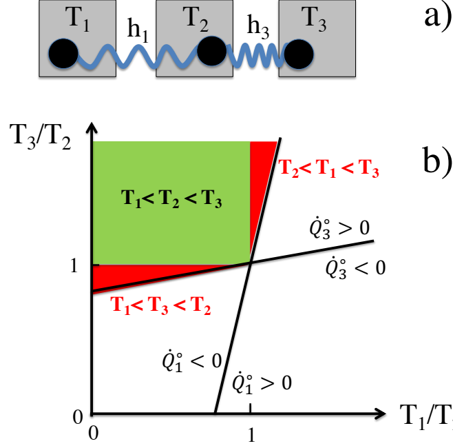
FIG. 2. a) Schematic representation of three particles that interact elastically and that are coupled to heat baths with different temperatures. b) Stationary heat flux diagram for symmetric elastic couplings h_1 = h_3 , showing a colored region where heat flows from particle 3 to particle 2, i.e. \dot{Q}_3^\circ > 0 , and heat flows from particle 2 to particle 1, i.e. \dot{Q}_1^\circ < 0 . The green area denotes the temperature range T_1 < T_2 < T_3 and the red areas denote T_2 < T_1 < T_3 and T_1 < T_3 < T_2 . The green area is the expected temperature range where heat flows from particle 3 coupled to the hot reservoir at T_3 to particle 2 coupled to the warm reservoir at T_2 and from particle 2 coupled to the warm reservoir at T_2 to particle 1 coupled to the cold reservoir at T_1 . In the red areas heat flows between the particles against the temperature gradients of the heat reservoirs: In the upper red area heat flows from particle 2 coupled to the cold reservoir at T_2 to particle 1 coupled to the warm reservoir at T_1 , in the lower red area heat flows from particle 3 coupled to the warm reservoir at T_3 to particle 2 coupled to the hot reservoir at T_2 .
