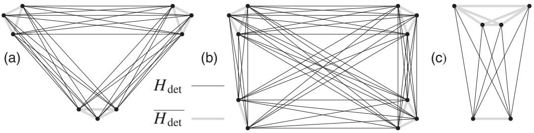
FIGURE 1 Some examples of the graphs H_{\det} and \overline{H_{\det}} from Definition 4.1 for each case: 1. (a) r = 9, k = q = r^* = 3 , 2. (b) r = 11, k = 3, q = 2, r^* = 4 , 3. (c) r = 6, k = 4, q = r^* = 2
