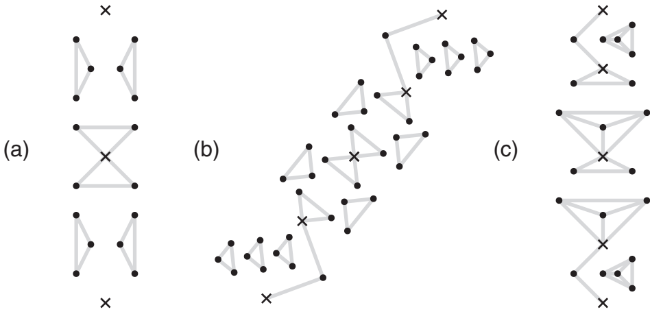
FIGURE 6 Some examples of H -paths for various H (see Definition 6.4 and Propositions 6.6,6.7 and 6.12 for relevant definitions): 1. (a) An \overline{H}_1 path with r=9 and k=q=r^*=3 . 2. (b) An \overline{H}_2 path with r=11, k=3, q=2 and r^*=4 . 3. (c) An \overline{H}_3 -path where H_3 = (H_0, H'_0, H'_0, H_0) \in \mathcal{H}_3 and we have r=6, k=4 and q=r^*=2
