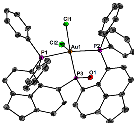
Figure 1. Molecular structure of (6-Ph 2 P-Ace-5-) 2 P(O)AuCl 2 ( 1 ) showing 50% probability ellipsoids and the essential atomic numbering. Selected bond parameters [Å, °]: Au1–P1 2.345(2), Au1–P2 2.365(1), Au1–P3 2.298(2), Au1–Cl1 2.392(2), Au1–Cl2 2.830(2), P3–O1 1.483(4), P1–Au1–P2 164.1(1), P1–Au1–P3 92.9(2), and P2–Au1–P3 82.8(2).
