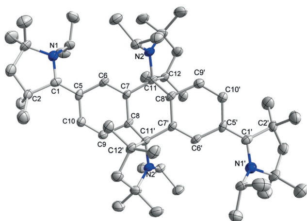
Figure 8. Molecular structure of 4^m_2 with thermal ellipsoids at 50%. All hydrogen atoms are omitted for clarity. Selected bond lengths [ \text{\AA} ] and bond angles [ ^\circ ]: N1–C1 1.391(5) , C1–C5 1.370(6) , C5–C6 1.465(6) , C6–C7 1.341(5) , C7–C8 1.512(6) , C8–C9 1.501(6) , C9–C10 1.336(6) , C10–C5 1.443(6) , C7–C11 1.535(6) , C8–C11' 1.594(5) , C11–N2 1.478(5) ; N1–C1–C2 109.33(30) , N2–C11–C12 103.00(26) .
