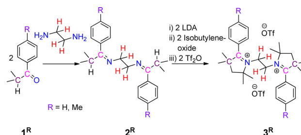
Scheme 2. Synthesis of N,N' -ethylene bridged bis-2-aryl pyrrolinium salts 3 R .
