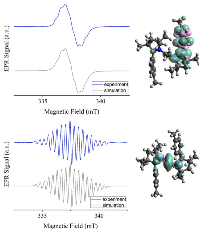
Figure 3. Left: Experimental (blue) and simulated (grey) EPR spectra of electrochemically generated 4^{Me} (top) and 7^{Me} (bottom). Right: calculated spin densities for 4^{Me} (top) and 7^{Me} (bottom).
