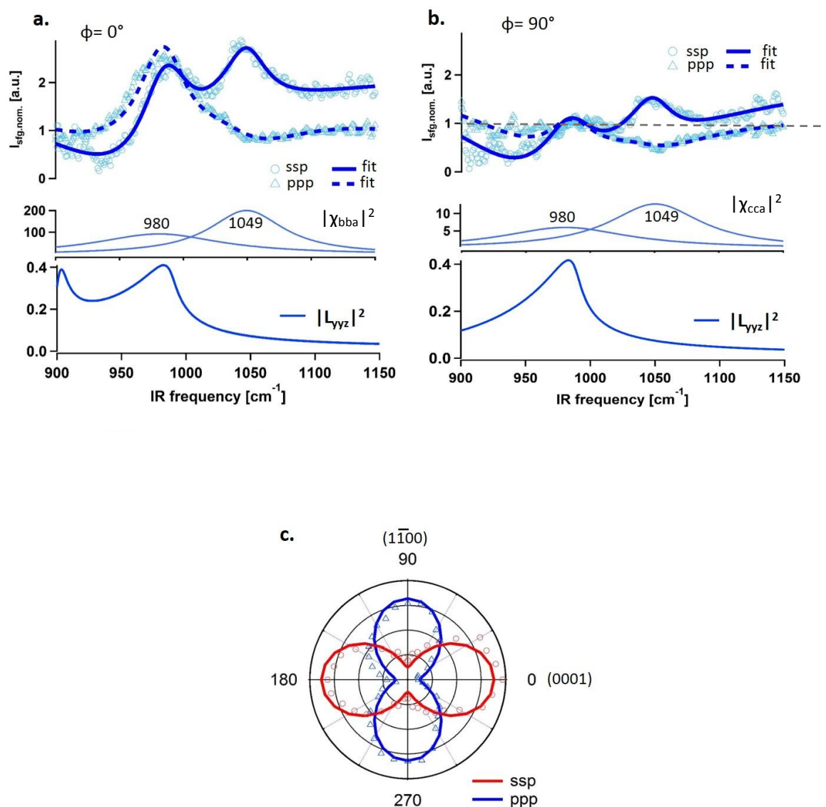
Figure 5. 10 SFG spectra of Al-O vibrations of \alpha -Al 2 O 3 (11-20) in ambient of sample 1: a) both ppp and ssp spectra collected at azimuthal angle \phi=0^\circ ; b) both ppp and ssp spectra collected at azimuthal angle \phi=90^\circ ; c) integrated I_{\text{sfg}} versus azimuthal orientation \phi of the sample for the feature at higher frequency (region from 1010 \text{cm}^{-1} to 1090 \text{cm}^{-1} ) in both ssp (red) and ppp (blue) spectra; All the spectra are collected at room temperature in ambient.
