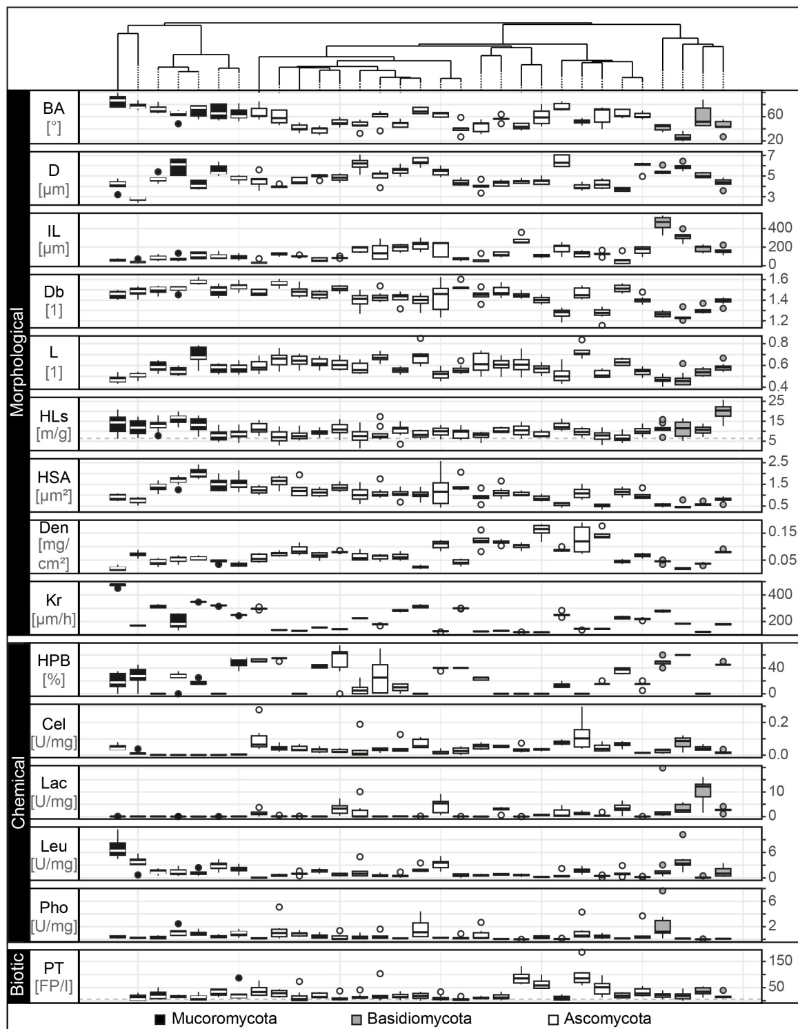
FIGURE 3 | Trait distributions. Tukey boxplots of the 15 trait variables comprising morphological, chemical and biotic fungal features. Here, we present data on branching angle (BA with n = 5 in ^{\circ} ), hyphal diameter (D with n = 5 in \mu\text{m} ), internodal length (IL with n = 5 in \mu\text{m} ), box counting dimension (Db with n = 8 , unitless), lacunarity (L with n = 8 , unitless), hyphal length in soil (HLS with n = 10 in \text{m/g} ), hyphal surface area (HSA with n = 8 in \mu\text{m}^2 ), biomass density (Den with n = 6 in \text{mg} \times \text{cm}^{-2} ), radial colony extension rate (Kr with n = 5 in \mu\text{m} \times \text{h}^{-1} ), hydrophobicity of fungal surfaces (HPB with n = 6 in % of ethanol molarity), cellobiohydrolase (Cel), laccase (Lac), leucine aminopeptidase (Leu), and acid phosphatase (Pho) activity (each with n = 5 in \text{unit} \times \text{g}^{-1} dry mass) and palatability (PT with n = 8 in no. of fecal pellets per collembolan individual). The boxplots represent 25th and 75th percentile, median and outlying points. Information about phylum affiliation is color-coded (black: Mucoromycota, gray: Basidiomycota, white: Ascomycota). The gray dashed line for the trait hyphal length in soil represents mean of corresponding trait controls. The trait database is available in Supplementary Table S6 .
