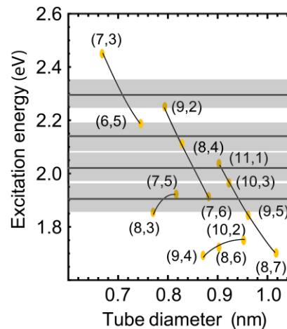
Figure 6 Kataura plot showing the excitation energy as a function of CNT diameter enabling to identify the accessible CNTs in e-TERS with the four chosen excitation wavelengths (grey markings).
