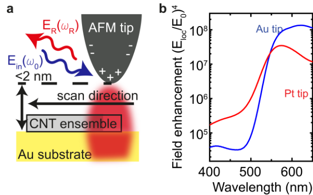
Figure 2a Principle of e -TERS. The incoming laser light illuminates the metallic tip and excites a near-field between tip and substrate. The strongly localized near-field drives the Raman process, i.e. it stimulates the sample and enhances the incoming and Raman scattered light. b Finite-difference time-domain simulation of the wavelength dependent field enhancement (E_{loc}/E_0)^4 between a PtIr-coated tip (red) and an Au tip (blue) above an Au substrate with 4 nm distance.
