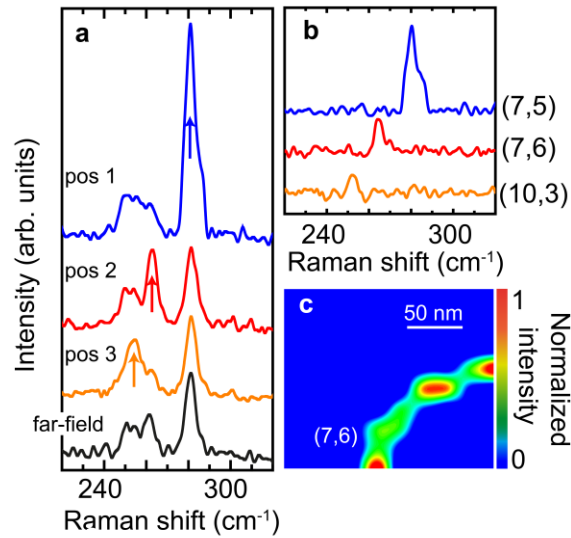
Figure 5a Composed spectra recorded at three different positions of the AFM tip. b pure TER spectra of three different RBMs, obtained by subtracting the far-field spectrum from the composed spectra. The tube species were assigned by the Raman shift of the appearing RBM. c Nanoimage of the (7,6) CNT.
