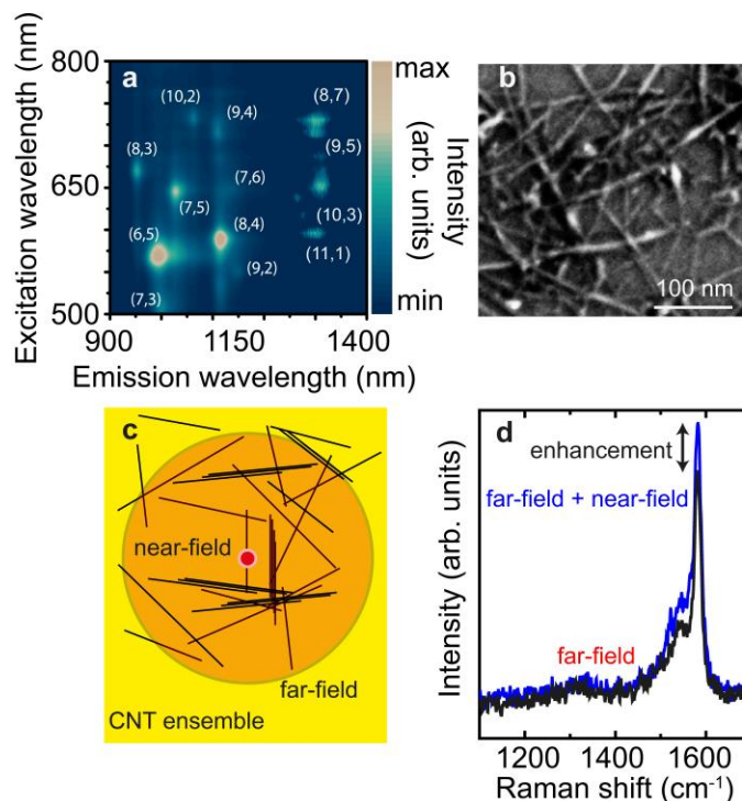
Figure 3a Photoluminescence excitation map of CNTs dispersed in an aqueous solution. The CNT species are indicated by the chiral indices. b Exemplary SEM image of the CNTs placed on an Au surface, c Scheme of the CNT ensemble that is stimulated by the near-field generated between tip and substrate (red dot) and the excitation laser (large red circle). d Composed near- (blue) and far-field Raman spectrum (black) of the characteristic G band of the CNTs.
