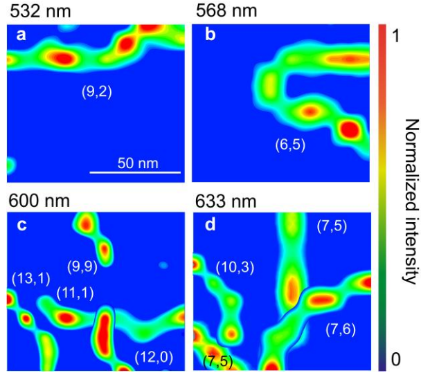
Figure 7 Nanoimages of the CNTs recorded with excitation wavelengths of (a) 532 nm, (b) 568 nm, (c) 600 nm and (d) 633 nm. The TER intensity of the RBMs is plotted as a function of tip position. The tube species were identified by their RBMs and labeled by the chiral indices in the nanoimages.
