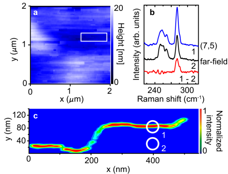
Figure 4a Topography image of a 2 x 2 μm CNT film. The position of the (7,5) in panel c is indicated by the white box. b Composed (blue), far-field (black) and TER spectra (red) of radial breathing modes of the (10,3), (7,6) and (7,5) species. c Nanoimage of the (7,5) CNT, obtained by plotting the tip enhanced RBM intensity as a function of tip position.
