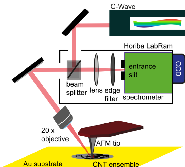
Figure 1 Scheme of the hyperspectral TERS setup. As a source of excitation energy, a fully tunable OPO laser is connected to a Horiba LabRam Raman spectrometer. The laser beam is guided through a beam splitter and focused by a 20x objective onto the tip apex of an AFM probe. The backscattered light is again collected by the objective. Raman spectra are recorded by guiding the tip-enhanced Raman scattered light of the sample via an edge filter into a grating spectrometer.
