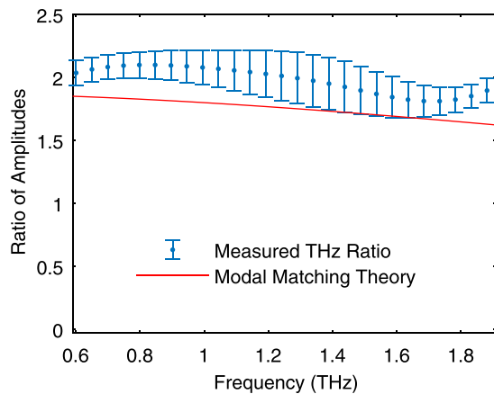
FIG. 3. Measured THz emission enhancement for different THz spectral components, plotting the THz field amplitude emitted from a spintronic trilayer with the dielectric cavity divided by field emitted without cavity, when excited by a pump pulse of 1040 nm. The solid line is a calculation from modal matching theory.
