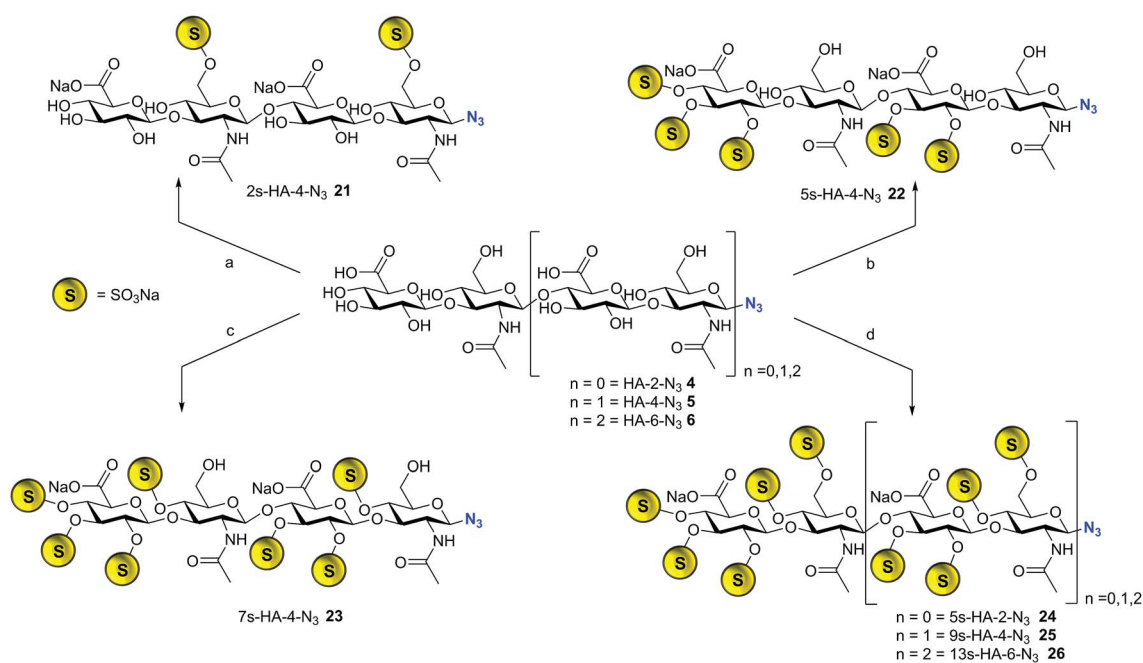
Scheme 2 Synthesis of selectively sulfated oligohyaluronan azides. Reaction conditions (a) \text{SO}_3 -Py, DMF, 0 °C, 1 h, 35%; (b) (i) \text{PhB}(\text{OH})_2 , DMF, 80 °C, 4 h; (ii) \text{SO}_3 -Py, 60 °C, 1 h, 45%; (c) (i) DMTrt-Cl, Py, 85 °C, 48 h; (ii) \text{SO}_3 -Py, 40 °C, 4 h, (iii) HFIP, water/ \text{CHCl}_3 , 38%; (d) \text{SO}_3 -Py, DMF, 6 h, 72% ( 24 ) 6 h, 74% ( 25 ) 6 h, 83% ( 26 ); DMTrt-Cl = 4,4'-dimethoxytriphenylmethyl chloride, HFIP = 1,1,1,3,3,3-hexafluoro-2-propanol.
