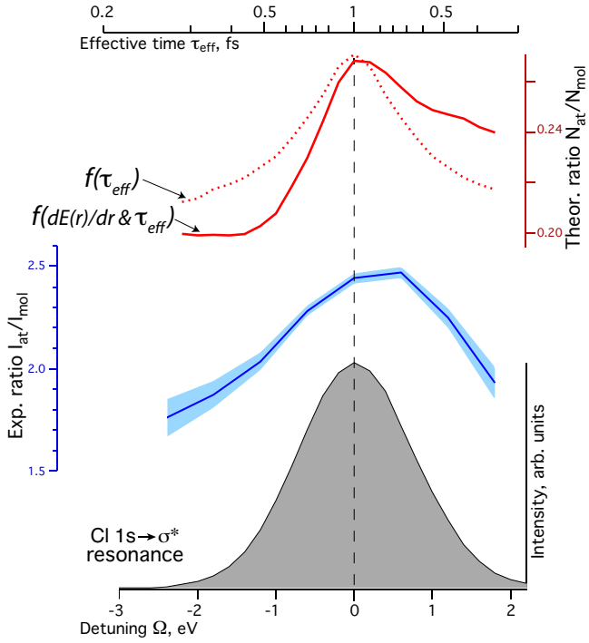
FIG. 2: Middle (in blue): experimental atomic-versus-molecular intensity ratio for MUST UFD in the Cl 2p^{-2}\sigma^* double-core-hole state of HCl following Cl 1s \rightarrow \sigma^* excitation using photon energies across the Cl 1s^{-1}\sigma^* resonance. Top (in red): theoretical atomic-versus-molecular ratio (including both \tau_{eff} and dE(r)/dr – full line; only \tau_{eff} – dotted). Error bars are indicated by shaded areas. Bottom: Cl 1s \rightarrow \sigma^* partial electron yield spectrum (equivalent to X-ray absorption).
