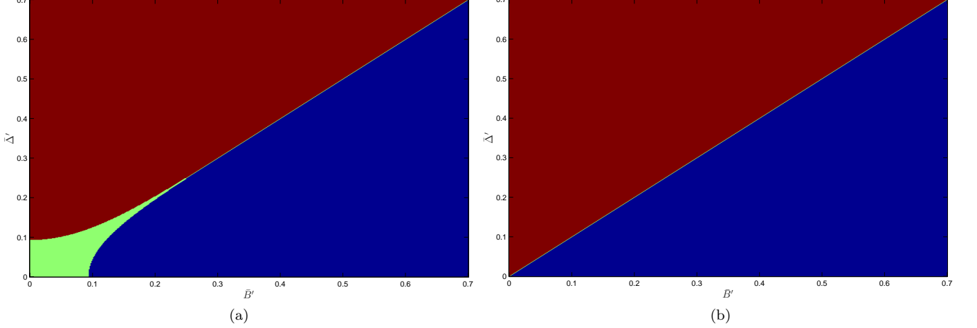
FIG. 4: The phase diagrams for (a) \epsilon = 0.2 and (b) \epsilon = -0.2 . The red region corresponds to a \Delta -dominated phase, the blue region corresponds to a B -terms phase, and the green regions correspond to gapless states.
