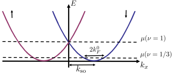
FIG. 2: The spectrum of an individual wire in the absence of interactions, Zeeman field, and proximity coupling. The dashed lines specify the chemical potentials corresponding to the situations \nu = 1 and \nu = 1/3 .
