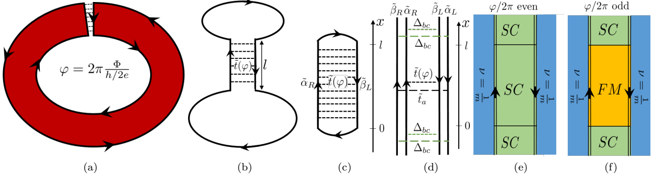
FIG. 3: A schematic depiction of the line of arguments used in order to identify the zero-modes localized at the center of h/2e vortices. (a) We start by placing our FCSC phase in an annular geometry, through which a magnetic flux may be inserted. Without altering the essential characteristics of the system, we cut a thin trench through the annulus. (b) As the presence of zero-modes should not depend on the precise geometry as long as the topological structure is preserved, we focus on the edge theory and fold our system inside-out to a bone shaped geometry. (c) The independence on the precise geometry allows us to shrink the outermost regions. (d) We examine an auxiliary model which has twice as many degrees of freedom, but whose low energy sector coincides with our model. We then show that the auxiliary model in (d) can be adiabatically deformed into a system composed of \nu = 1/m fractional quantum Hall edges coupled by ferromagnetic and superconducting terms. (e) If the flux \varphi is an even multiple of 2\pi , we get effective superconducting term throughout the system, meaning there are no zero modes. (f) For odd multiples of 2\pi , the superconductor in the physical region is replaced by a ferromagnet. The domain walls of the resulting configuration, representing the edges of the original configurations, give rise to parafermionic bound states [37–39].
