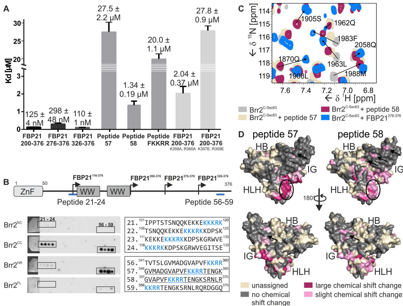
Figure 3. The interaction between FBP21 and Brr2 is partly mediated by a positively charged peptide contained in FBP21's C-terminal region. (A) Dissociation constants of FBP21 fragments and Brr2 C-Sec63 were determined by ITC. Shown are average K_D values and standard deviations derived from three experiments each. (B) Domain organization of FBP21 as in 1A. Blue bars show the location of the peptides interacting with Brr2 derived from the peptide SPOT analysis. Brr2 CC and Brr2 HR interacted with two regions on the SPOT membrane, both of which contained a positively charged stretch. (C) Excerpt of overlaid 1 H- 15 N-TROSY-HSQC spectra of 100 \mu\text{M} Brr2 C-Sec63 alone (gray) in presence of sevenfold excess of peptide 57 (beige), in presence of sevenfold excess of peptide 58 (dark pink) and in presence of a 4-fold excess of FBP21 276-376 (blue). Examples of differentially shifting peaks are shown. (D) The binding sites of peptide 57 and peptide 58 was determined by plotting residues with significant chemical shifts changes on the structure of Brr2 C-Sec63 (PDB ID 4F91). Unassigned residues are shown in beige, assigned residues that have no or non-significant chemical shift change are shown in dark gray. Residues exhibiting a chemical shift change upon interaction with the peptides are shown in pink as two categories. Dark pink denotes a chemical shift change above the average plus standard deviation of the chemical shift changes of all residues in the experiment ( \Delta\delta = 0.053 ppm and \Delta\delta = 0.109 ppm for peptide 57 and peptide 58, respectively), light pink denotes a chemical shift change above the average chemical shift change of all residues in the experiment ( \Delta\delta = 0.022 ppm and \Delta\delta = 0.040 ppm for peptide 57 and peptide 58, respectively). Circles indicate the negatively charged surface on the HLH domain that is contacted by all measured FBP21 fragments, arrows indicate residues with chemical shift changes outside of the likely binding site. For comparison of the binding sites of peptide 57, peptide 58 and FBP21 276-376 on Brr2 C-Sec63 , the residues with chemical shift changes are shown side-by-side using the same thresholds for all experiments in Supplementary Figure S8.
