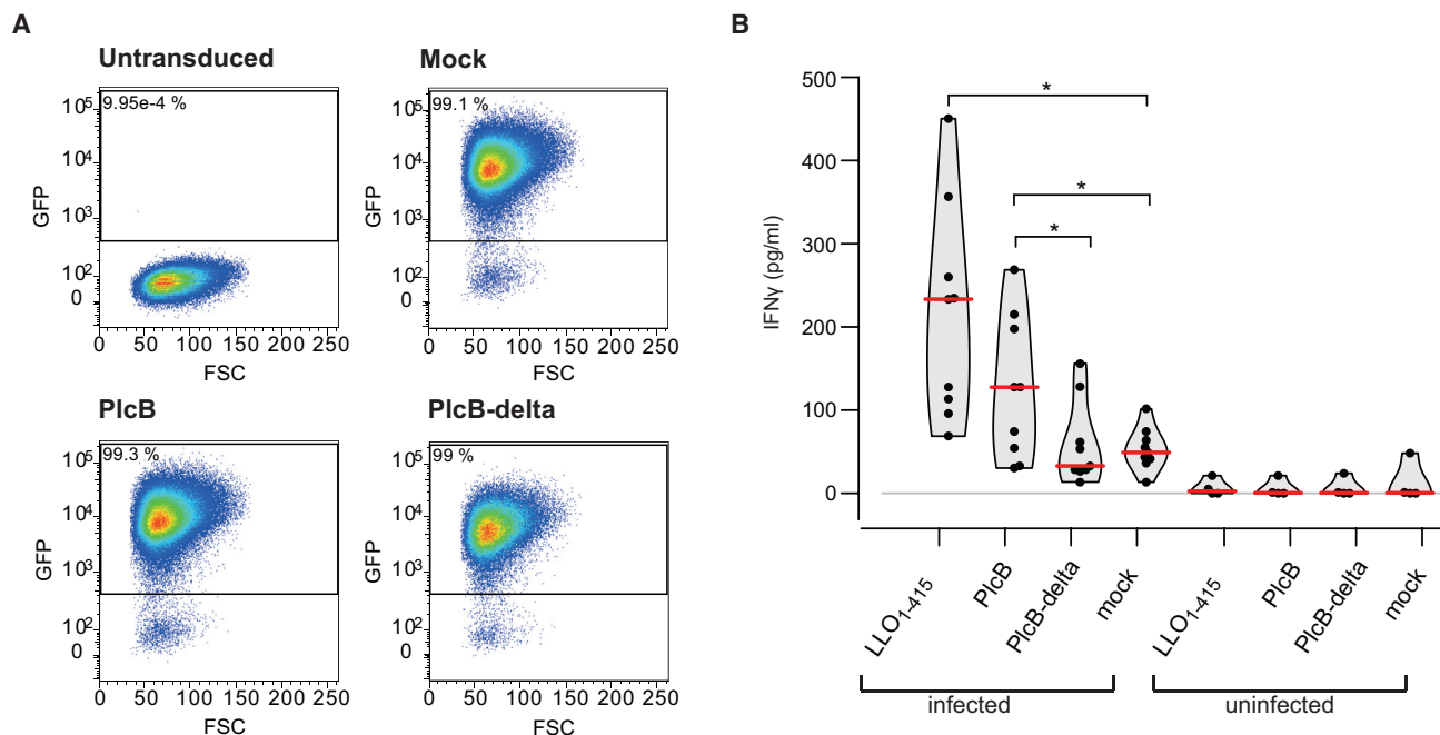
Figure 5. Identified PlcB-Spliced Epitopes Are Processed and Presented by EL4 Cells Expressing the L. monocytogenes -Derived PlcB Protein
