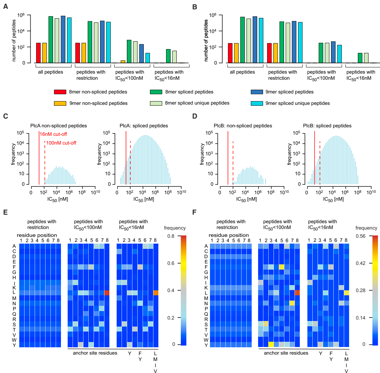
Figure 2. In Silico Identification of a Spliced Peptide Candidate List
