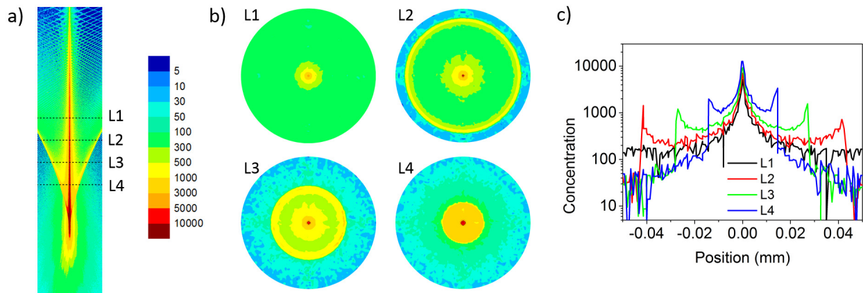
Figure 7. Optical simulations of hemispherical micro lens made from n = 1.5 material on such one: a) ray propagation, lines corresponding to distances of L1 = 1.5 mm, L2 = 1.6 mm, L3 = 1.7 mm and L4 = 1.8 mm from the lens (not to scale: y-range 1.3 mm, x-range 0.1 mm), b) concentration distributions in the different planes, spot diameter 100 \mu\text{m} (same color scale as in a), c) corresponding line profiles through the focal spots.
