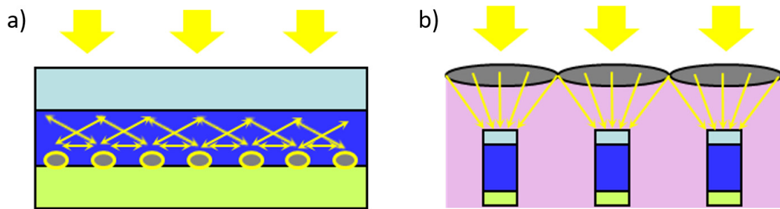
Figure 1. Concepts for material saving and efficiency enhancement in CIGSe solar cells: a) ultra-thin solar cell with integrated nanostructures for localizing light inside the absorber material, b) micrometer-sized solar cells under concentrated illumination due to the application of micro lenses.
