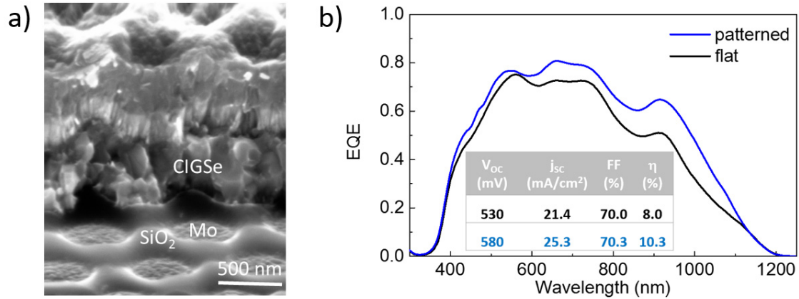
Figure 4. a) SEM cross-section of an ultra-thin CIGSe solar cell on top of a SiO 2 network, b) corresponding EQE as compared to planar reference.
