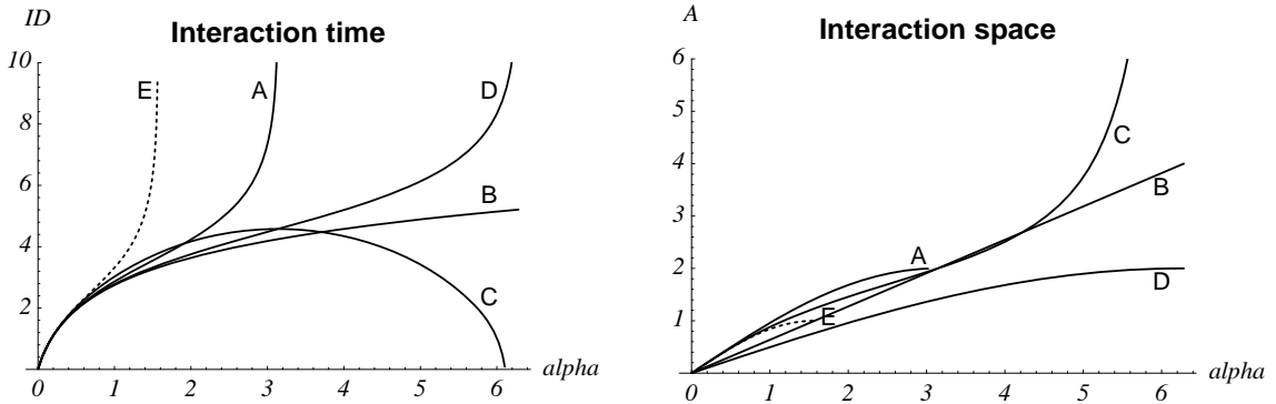
Figure 5: Interaction time is linear to the index of difficulty ID on the left—given for a fixed angular resolution of ten degree. The space needed for an interaction task of an angle \alpha is shown on the right. VIRTUAL-SPHERE-metaphor with synchronous movement (A), linear mapping (B), parabolic geometry (C), ARCBALL-metaphor (D), and VIRTUAL-SPHERE-metaphor with the movement model starting in the midpoint (E, dashed line).
