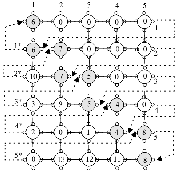
Figure 18 Lower triangularization
