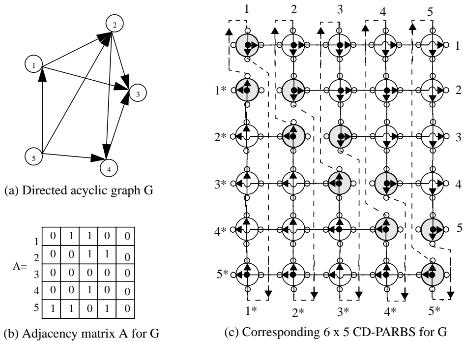
Figure 2 Embedding the directed acyclic graph in to a 6 x 5 CD-PARBS
