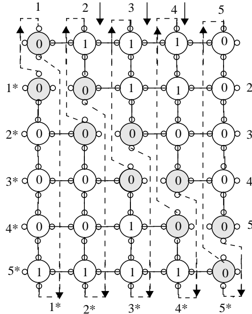
Figure 4 Each plane sends its transitive closure value to the first plane
