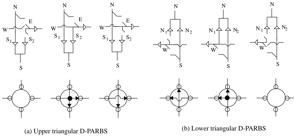
Figure 1 Processors and switches in D-PARBS
