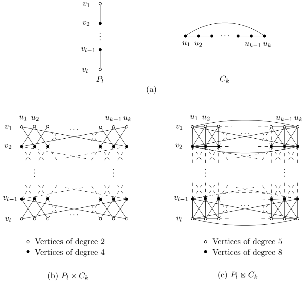
Figure 1. (a) Path graph on l vertices P_l , and cycle graph on k vertices C_k , (b) direct product graph P_l \times C_k , and (c) strong product graph P_l \boxtimes C_k .
