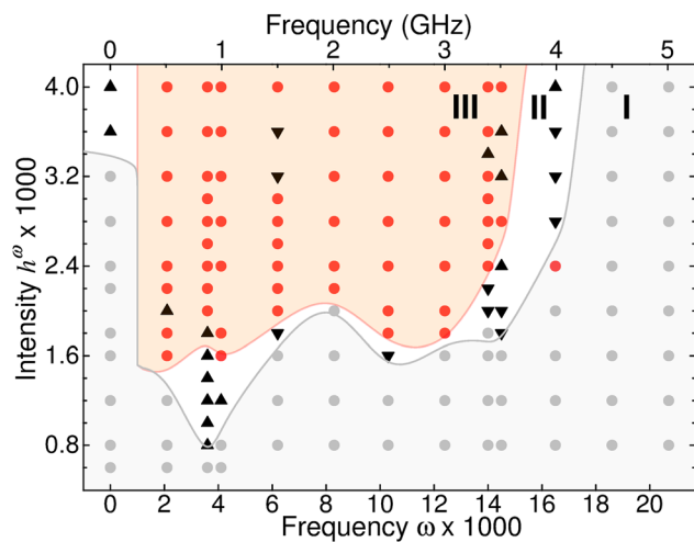
FIG. 4. Phase diagram of the skyrmion switching induced by a field h^\omega = h^\omega \sin(\omega t) as a function of h^\omega and \omega . Red dots indicate skyrmion reversal, gray dots mean no switching, up-pointing and down-pointing triangles skyrmion switching to uniform and distorted states, respectively.
