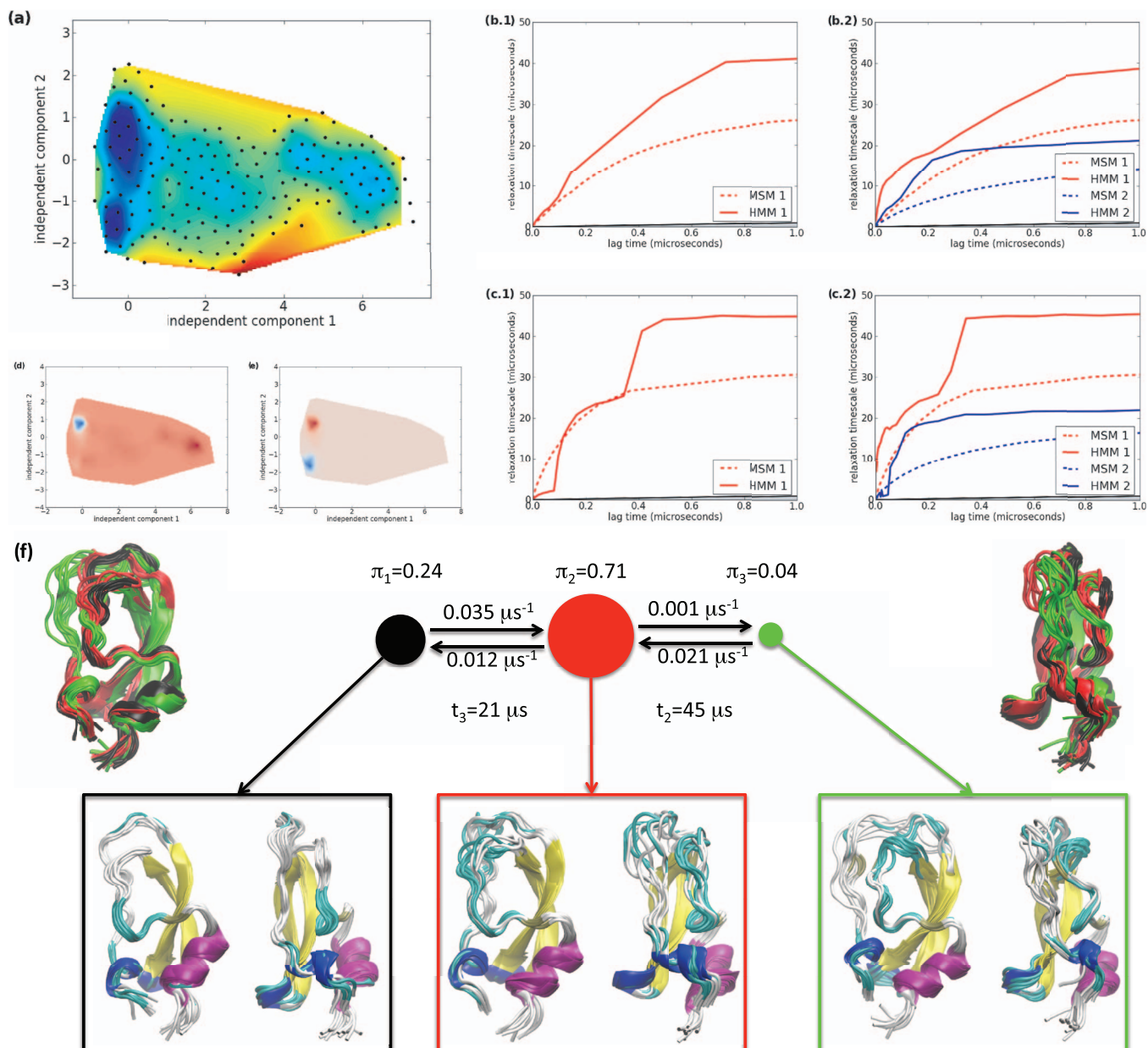
FIG. 3. Comparison of MSM and PMM/HMM for modeling the conformation dynamics of BPTI using a 1 ms simulation trajectory generated by the Anton supercomputer 37 and kindly provided by D.E. Shaw research. The discretization consisted of either 13 or 191 clusters, approximately uniformly distributed on the data projected onto the space of the two dominant independent components of a TICA analysis (see Ref. 27 for details), using the EMMA software implementation. 36 (a) 191 clusters and a visualization of their reduced free energy, -\ln \pi_i . (b) and (c) Comparison of the slowest MSM timescales with the timescales of the 2- and 3-states HMM, respectively, using 13 clusters ((b.1) and (c.1)) or 191 clusters ((b.2) and (c.2)). (d) and (e) Visualization of the second and third eigenvectors, \mathbf{l}_2 and \mathbf{l}_3 for the 191 cluster discretization. (f) Three-state rate matrix corresponding to the 3-state HMM. The structures are overlays of 10 frames drawn from the state distributions \chi_1 , \chi_2 , and \chi_3 .
