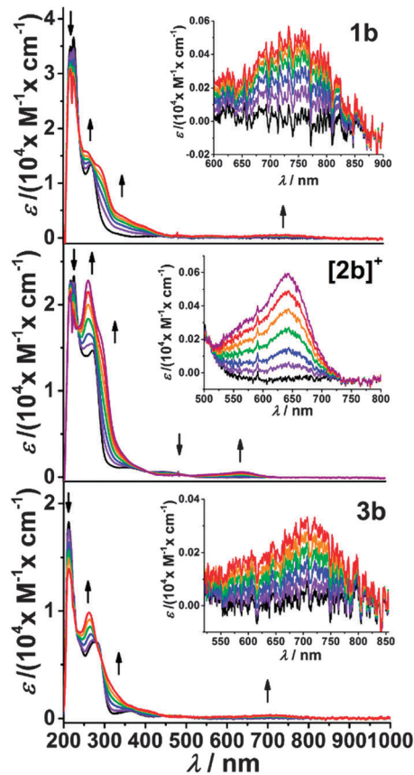
Fig. 4 Changes in the UV/Vis absorption of 1b , [2b]^+ and 3b in the course of a one-electron oxidation in THF/0.1 M Bu_4NPF_6 at room temperature. Insets show a zoom of the long wavelength band.
