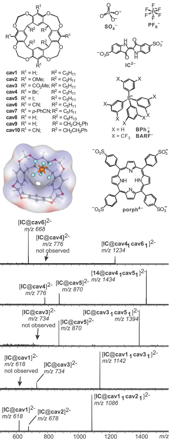
Fig. 12 Top, left: anion-binding cavitannds cav1 – cav10 and B3LYP/6-31++G(d,p)-optimized structure of complex [PF_6@cav1]^- with the electrostatic potential mapped on the host's van der Waals surface. Top, right: guest anions. Bottom: CID experiments with mass-selected, doubly charged heterodimeric IC^{2-} complexes. Adapted and reproduced from ref. 55 with kind permission by Wiley-VCH.
