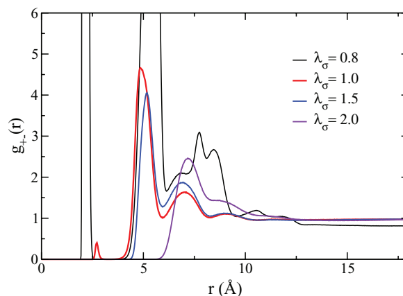
FIG. 11. Radial cation-anion distribution function g_{+-} for a 0.5 m \text{CaCl}_2 solution for different values of the scaling prefactor \lambda_\sigma . With increasing \lambda_\sigma the direct ion pair peak of the RDF decreases and the whole distribution shifts to larger cation-anion distances, which explains the increase of a_{cc} as \lambda_\sigma grows.
