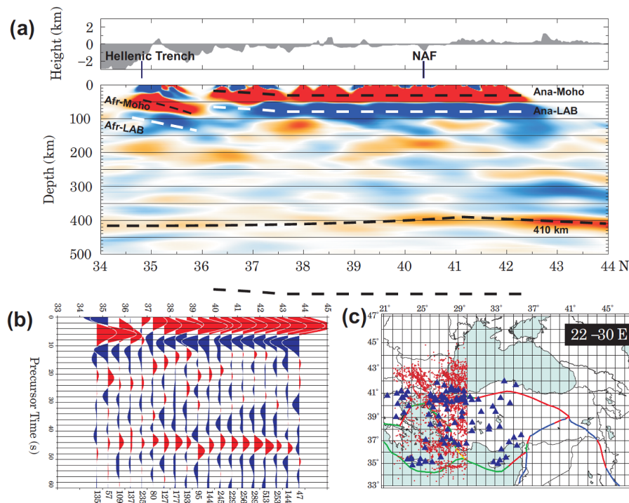
Figure 5. Display of S-receiver functions along a north–south profile between 22 and 30° E (Aegean and western Anatolia). Topography is displayed on top of the figure. (a) CCP stack (depth–transformation). (b) Time-domain stack for same profile as in (a) . A slowness of 6.4 \text{ s degree}^{-1} is used for the moveout correction. The binning is determined by the location of piercing points at 200 km depth. The numbers below the bottom y axis show how many traces have contributed to each trace. (c) Blue triangles are stations which contributed data to the profile. Red dots are locations of S-to-P piercing points at 200 km depth.
