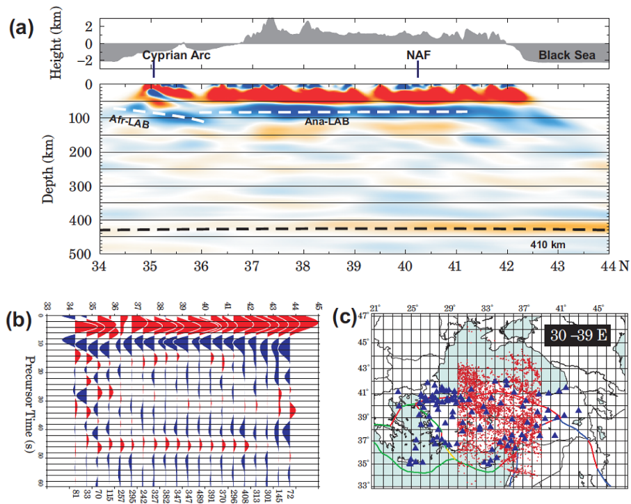
Figure 6. Same as Fig. 5 for a north–south profile between 30 and 39° E (central Anatolia). The width of this profile is too wide to see details of the subduction near Cyprus. See Fig. 8 for more details. No change in depth across the North Anatolian Fault is noticeable (NAF in a).
