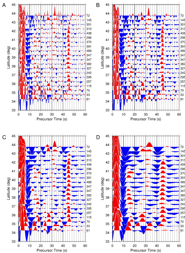
Figure 11. Same S-receiver functions as in Fig. 6b for different filters: (a) no filter, (b) 2 s low-pass filter, (c) 4 s low-pass filter and (d) 8 s low-pass filter. At shorter periods (a and b) the LAB (blue signal around 10 s) may consist of several smaller discontinuities. Only for the 6 and 8 s low-pass filters it appears as a single discontinuity. In contrast, the Moho and the discontinuity at 410 km depth (red signals around 5 and 45 s, respectively) remain as sharp single discontinuities at all periods, suggesting that this behavior is due to structure rather than to the higher noise levels at shorter periods.
