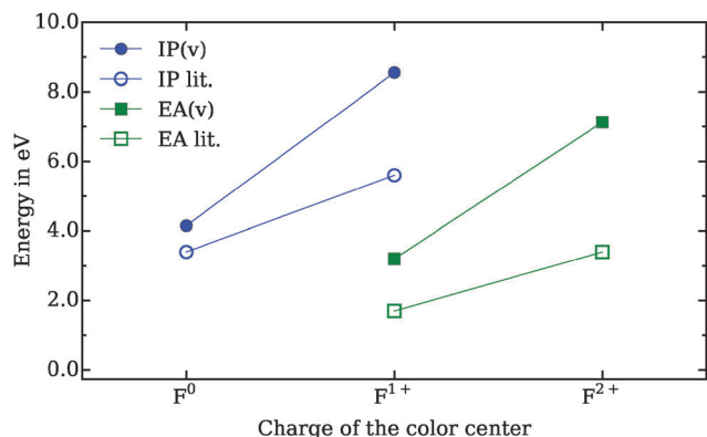
Fig. 3 Vertical ionization potential (IP) and electron affinity (EA) of F n → F n +1 + e - and F n + e - → F n -1 , respectively, compared to literature values. 36 Due to the restricted size and, as a consequence, restricted ability of polarization of the QM cluster, the deviation to the literature values increases with the number of electron holes. The lines serve as a guide to the eye.
